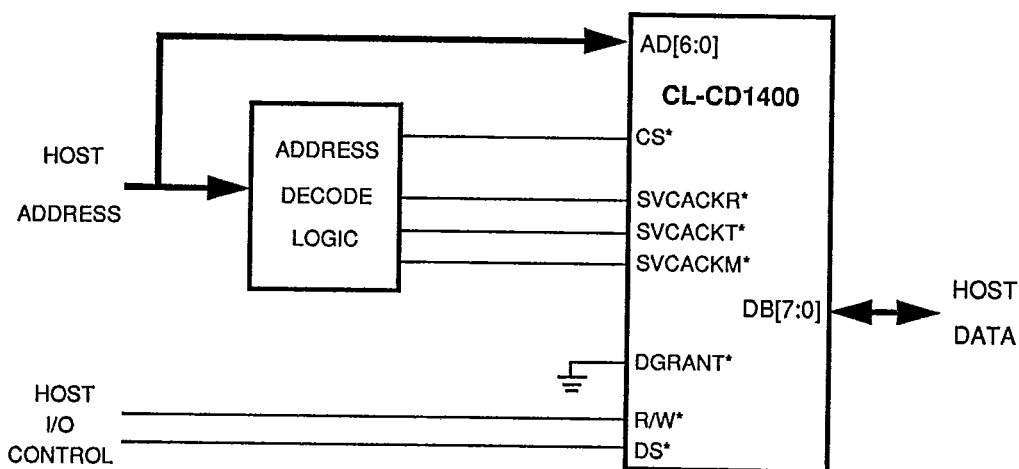
Figure 4-3. Control Signal Generation
