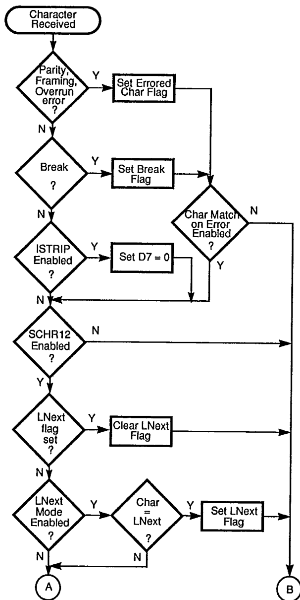
Figure 4-6. CL-CD1400 Receive Character Processing
