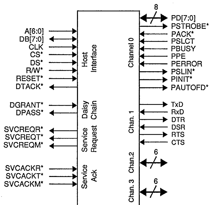
Pin Functions, Three Serial/One Parallel Channel Mode
