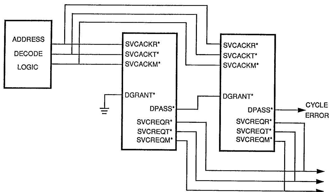
Figure 4-4. CL-CD1400 Daisy-Chain Connections
