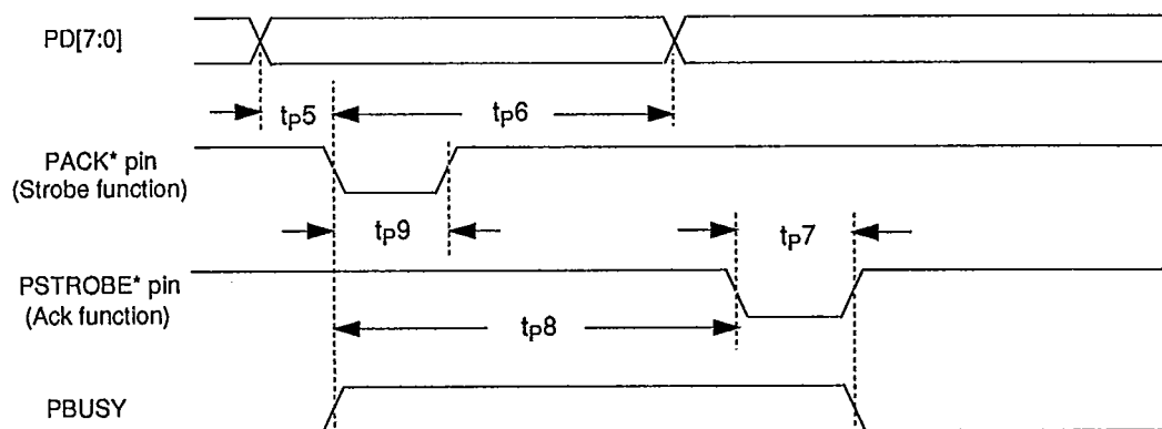
Figure 3-10. Parallel Port Receive Timing
