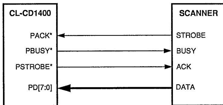
Figure 4-9. CL-CD1400 Parallel Data Receive Connections
