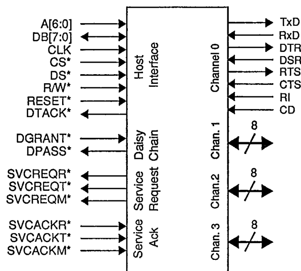
Pin Functions, Four Serial Channel Mode
