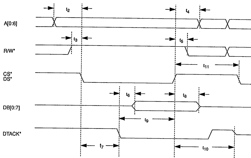
Figure 3-3. Asynchronous Read Cycle Timing
