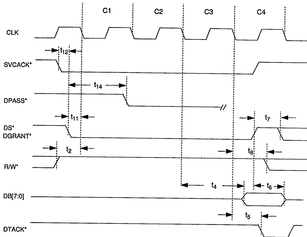
Figure 3-8. Synchronous Service Acknowledge Cycle Timing
