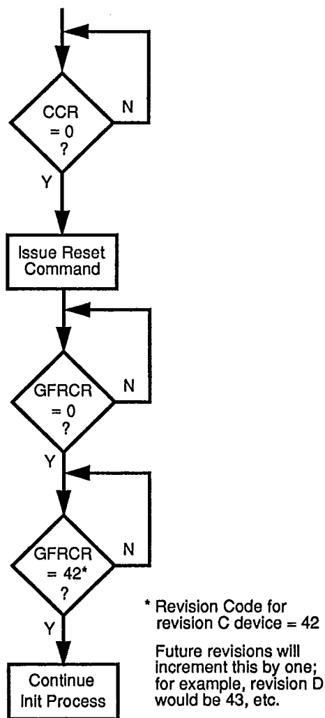
Figure 6-1. Flow Diagram of CL-CD1400 Master Initialization Sequence
