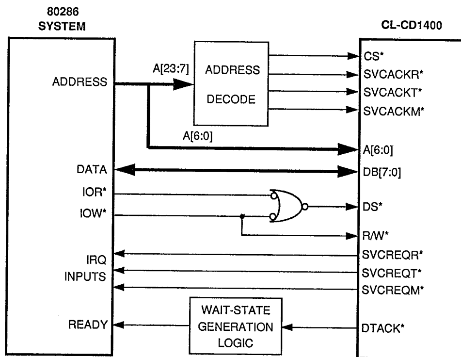
Figure 4-10. Intel 80x86 Family Interface
