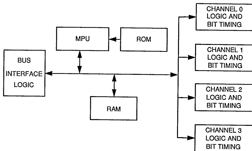
Figure 4-1. CL-CD1400 Functional Block Diagram
