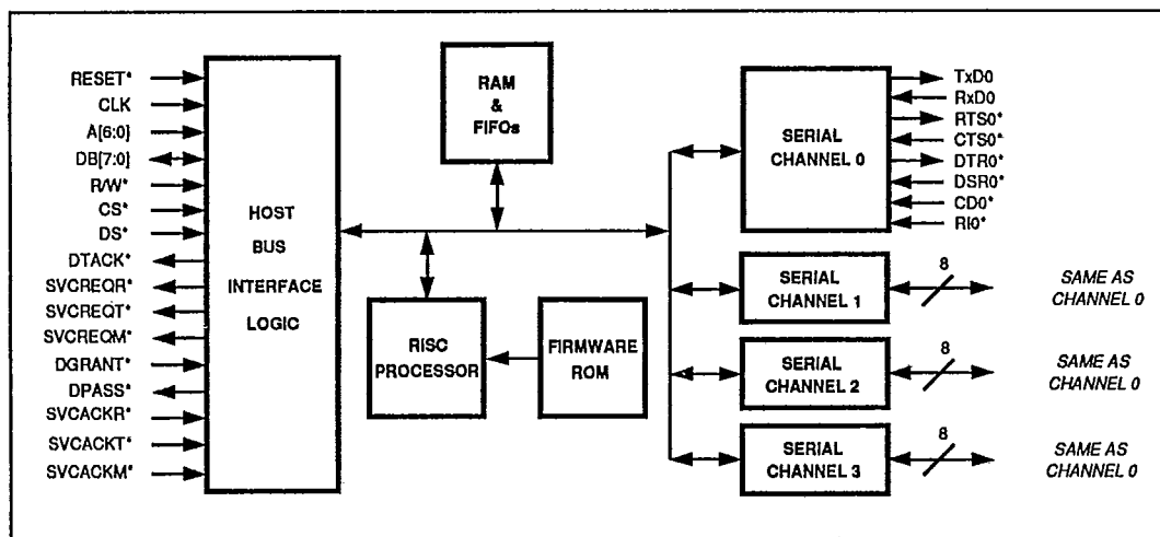
Figure 1-4. Four Full-Modem Ports
