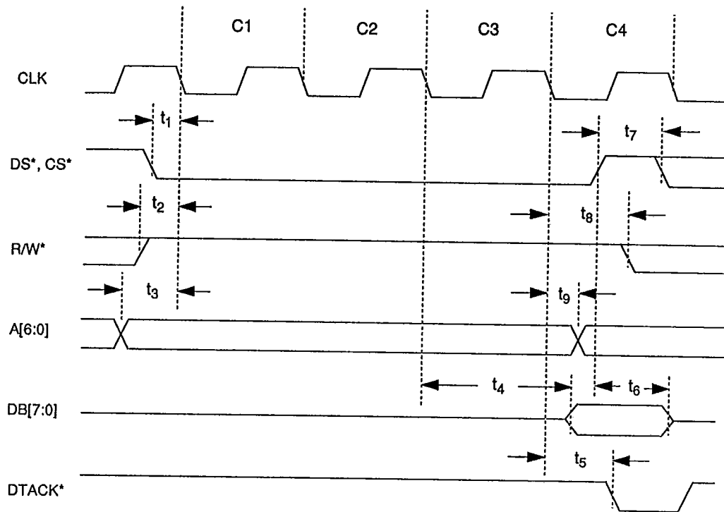
Figure 3-6. Synchronous Read Cycle Timing
