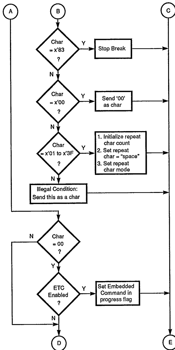
Figure 4-7. CL-CD1400 Transmit Character Processing (cont.)
