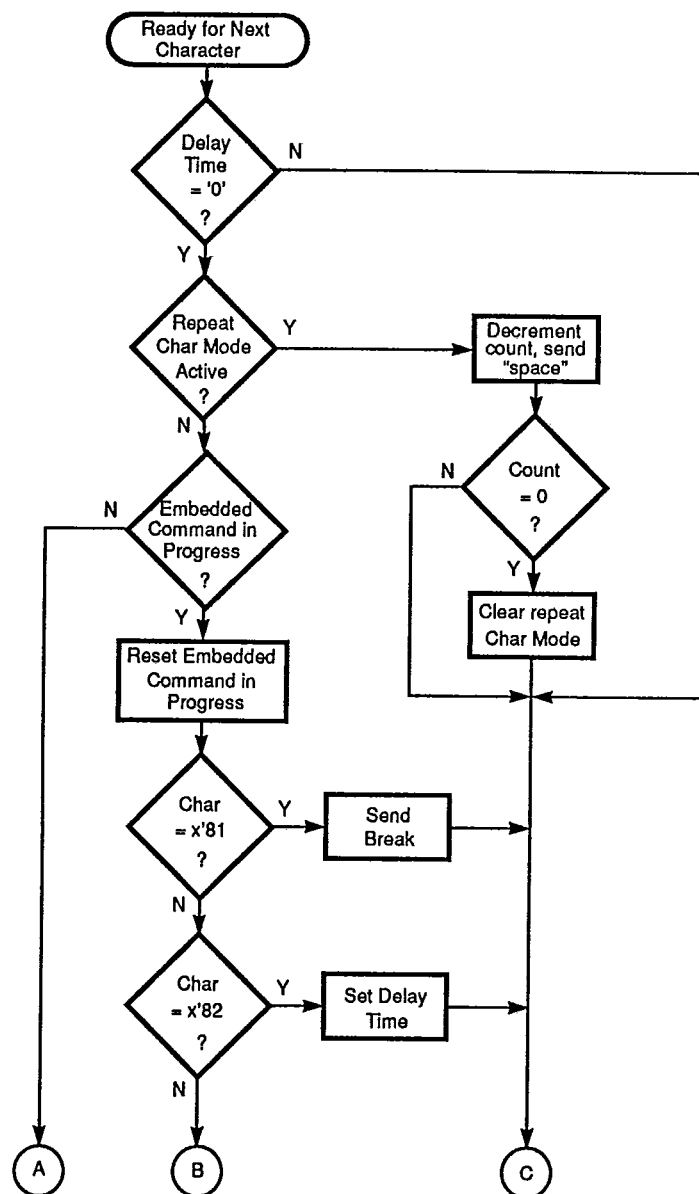
Figure 4-7. CL-CD1400 Transmit Character Processing
