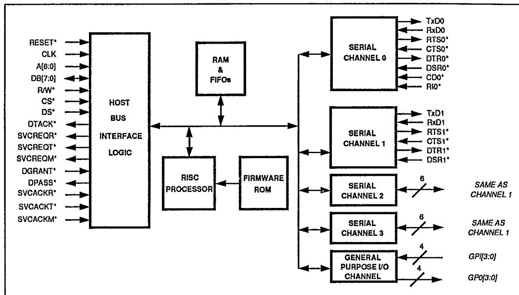
Figure 1-3. One Full-Modem Port, Three Serial Channels and One Eight-Bit I/O Port
