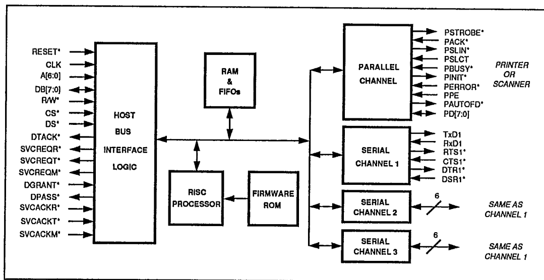
Figure 1-2. Three Serial Ports and One Parallel Port
