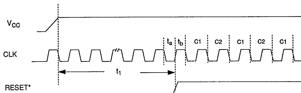
Figure 3-1. Reset Timing
