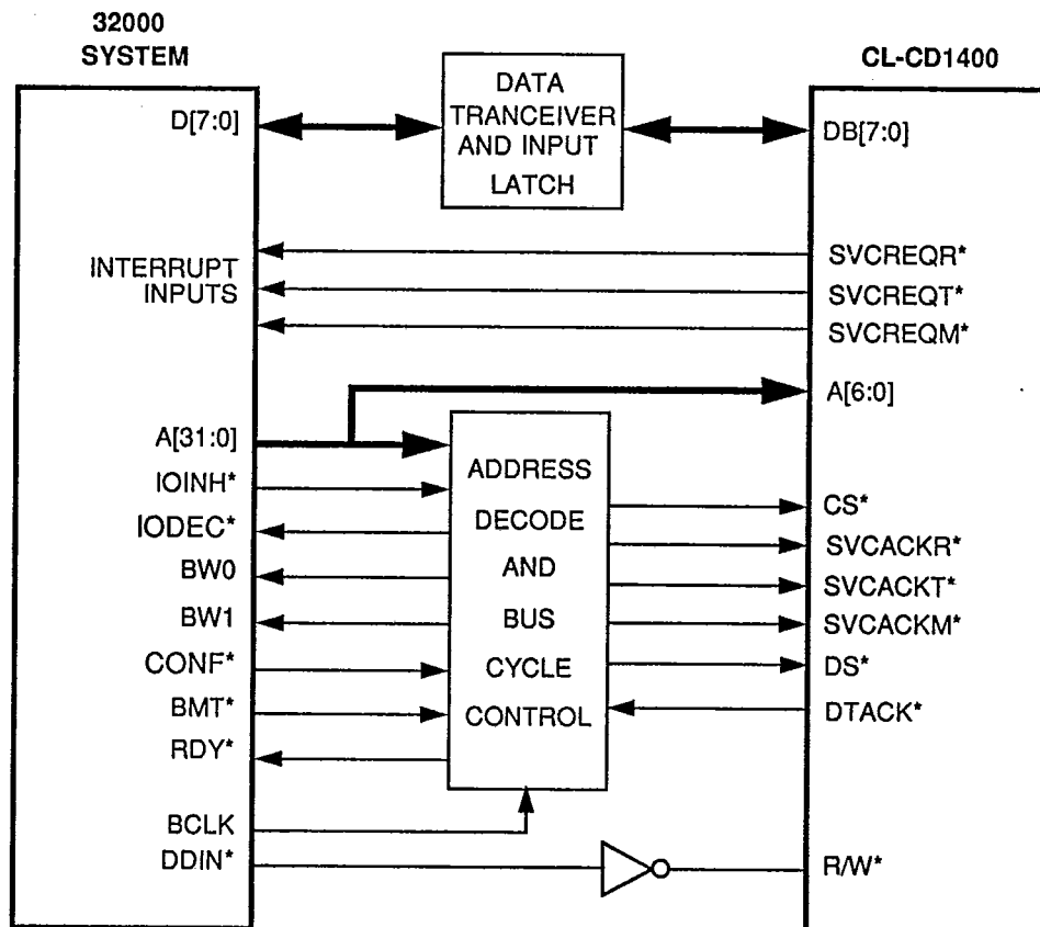
Figure 4-12. National 32000 Interface
