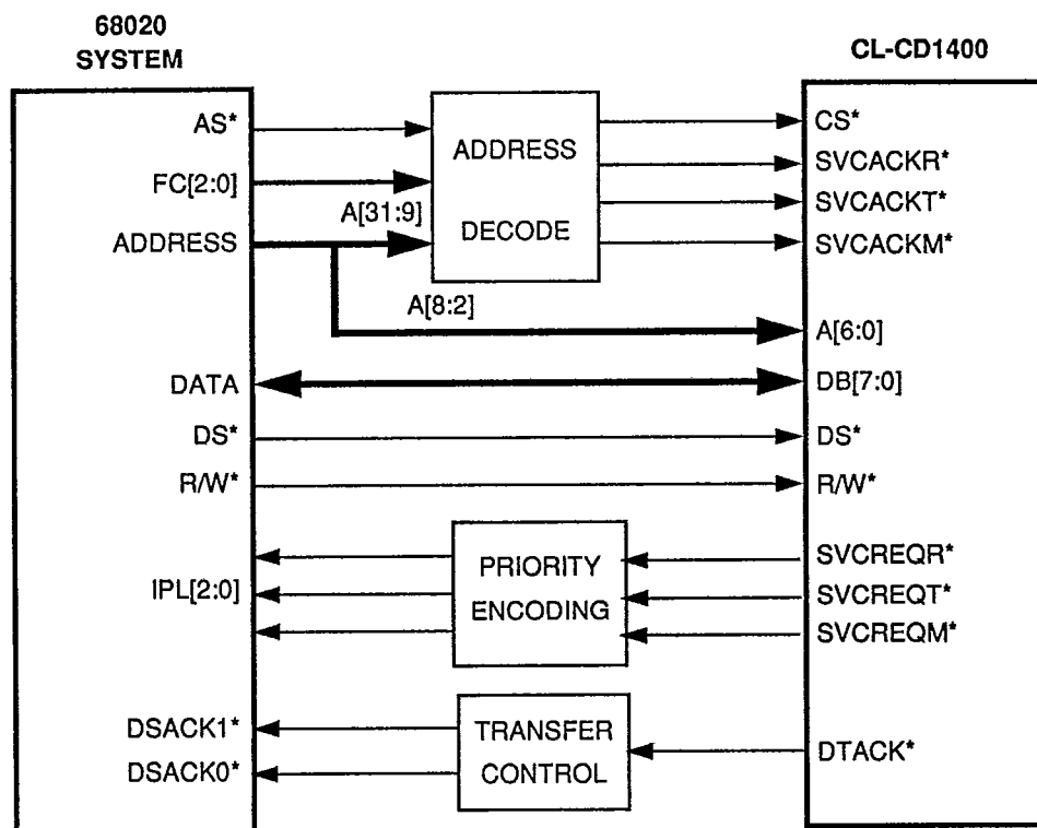
Figure 4-11. Motorola 68020 Interface
