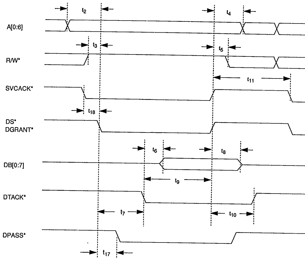
Figure 3-5. Asynchronous Service Acknowledge Cycle Timing
