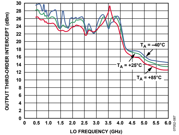
Figure 18. OIP3 vs. LO Frequency ( f_{LO} ) and Temperature ( P_{OUT} \approx -5 dBm @ f_{LO} = 900 MHz)
