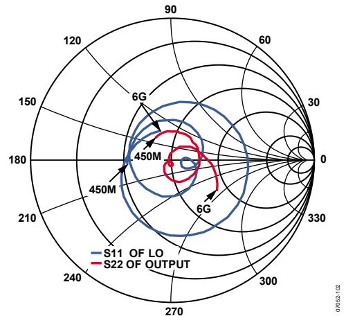
Figure 32. Smith Chart of LOIP (LOIN AC-Coupled to Ground) S_{11} and RFOUT S_{22} from 450 MHz to 6000 MHz
