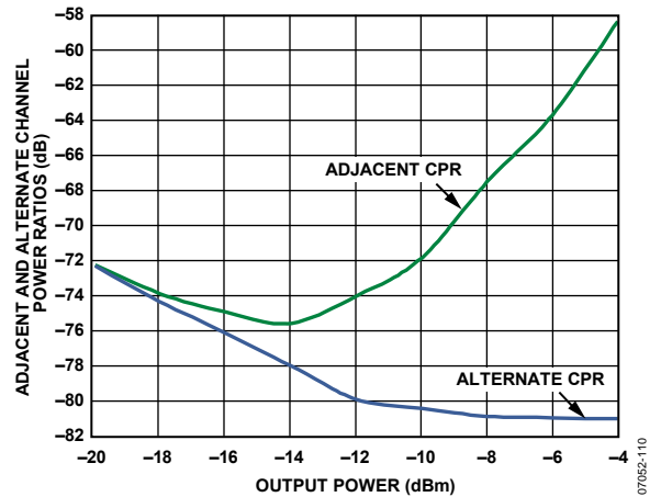
Figure 67. ADL5375-15 Single-Carrier W-CDMA Adjacent and Alternate Channel Power vs. Output Power at 2140 MHz; LO Power = 0 dBm
