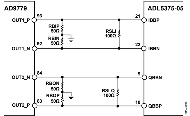
Figure 58. AC Voltage Swing Reduction Through the Introduction of a Shunt Resistor Between Differential Pair
