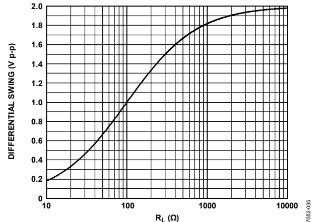
Figure 59. Relationship Between the AC Swing-Limiting Resistor and the Peak-to-Peak Voltage Swing with 50 Ω Bias-Setting Resistors
