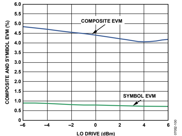
Figure 68. ADL5375-05 Single Carrier W-CDMA Composite and Symbol EVM vs. LO Drive at 2140 MHz; Output Power = -10 dBm
