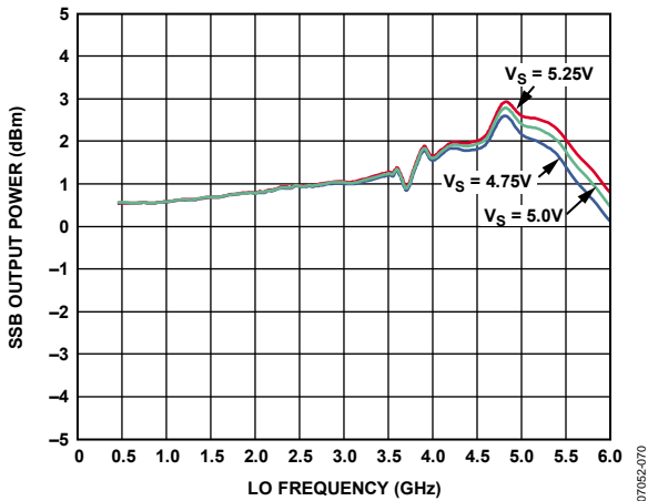
Figure 29. Single-Sideband (SSB) Output Power ( P_{\text{out}} ) vs. LO Frequency ( f_{\text{LO}} ) and Supply
