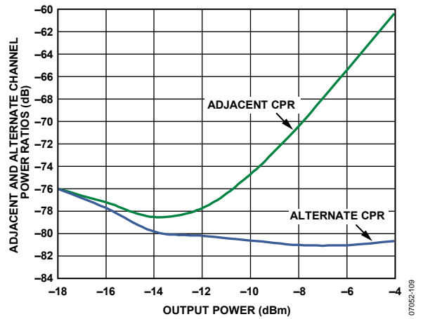
Figure 66. ADL5375-05 Single-Carrier W-CDMA Adjacent and Alternate Channel Power vs. Output Power at 2140 MHz; LO Power = 0 dBm
