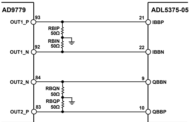
Figure 57. Interface Between the AD9779 and ADL5375-05 with 50 Ω Resistors to Ground to Establish the 500 mV DC Bias for the ADL5375-05 Baseband Inputs
