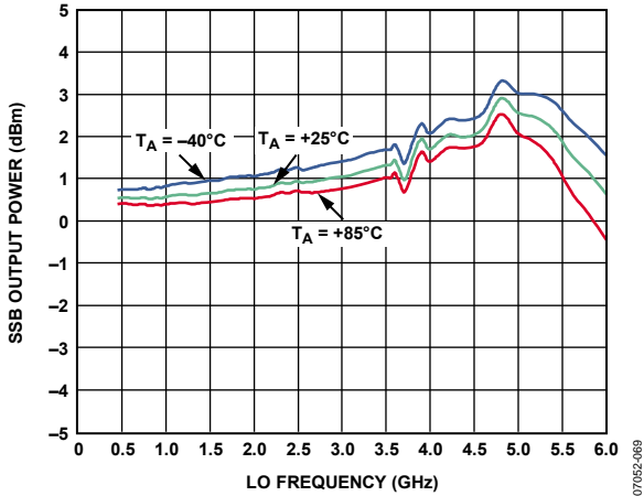
Figure 28. Single-Sideband (SSB) Output Power ( P_{\text{out}} ) vs. LO Frequency ( f_{\text{LO}} ) and Temperature
