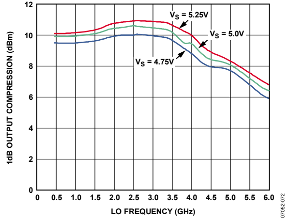
Figure 31. SSB Output 1dB Compression Point ( OP_{1\text{dB}} ) vs. LO Frequency ( f_{\text{LO}} ) and Supply
