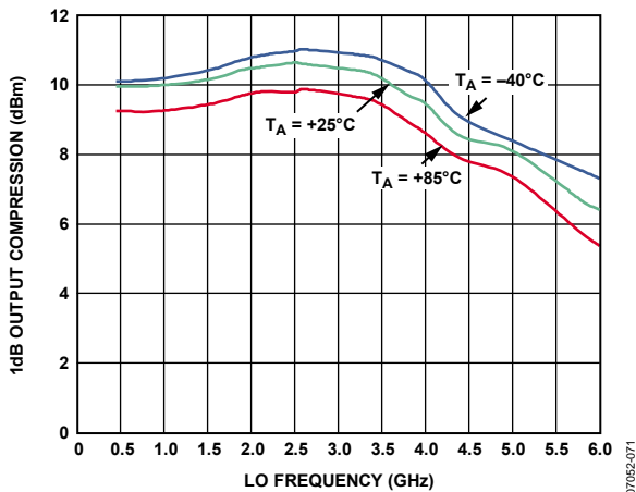
Figure 30. SSB Output 1dB Compression Point ( OP_{1\text{dB}} ) vs. LO Frequency ( f_{\text{LO}} ) and Temperature
