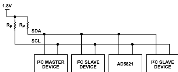
Figure 21. Typical I 2 C Bus
