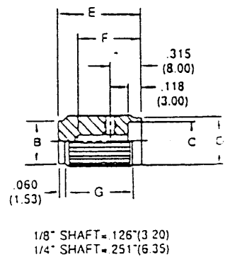
CONTROL KNOB WITH STRAIGHT KNURL AND TOP LINE INDICATOR
