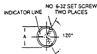
CONTROL KNOB WITH STRAIGHT KNURL AND TOP LINE INDICATOR
