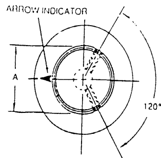
STRAIGHT KNURL WITH ARROWHEAD INDICATOR ON SKIRT
