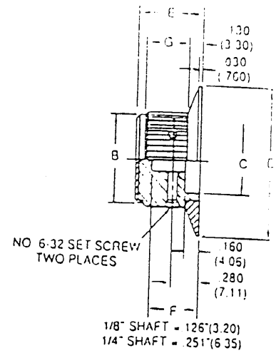
STRAIGHT KNURL WITH ARROWHEAD INDICATOR ON SKIRT
