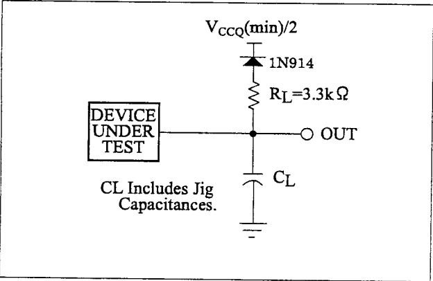
Figure 6. Transient Equivalent Testing Load Circuit
