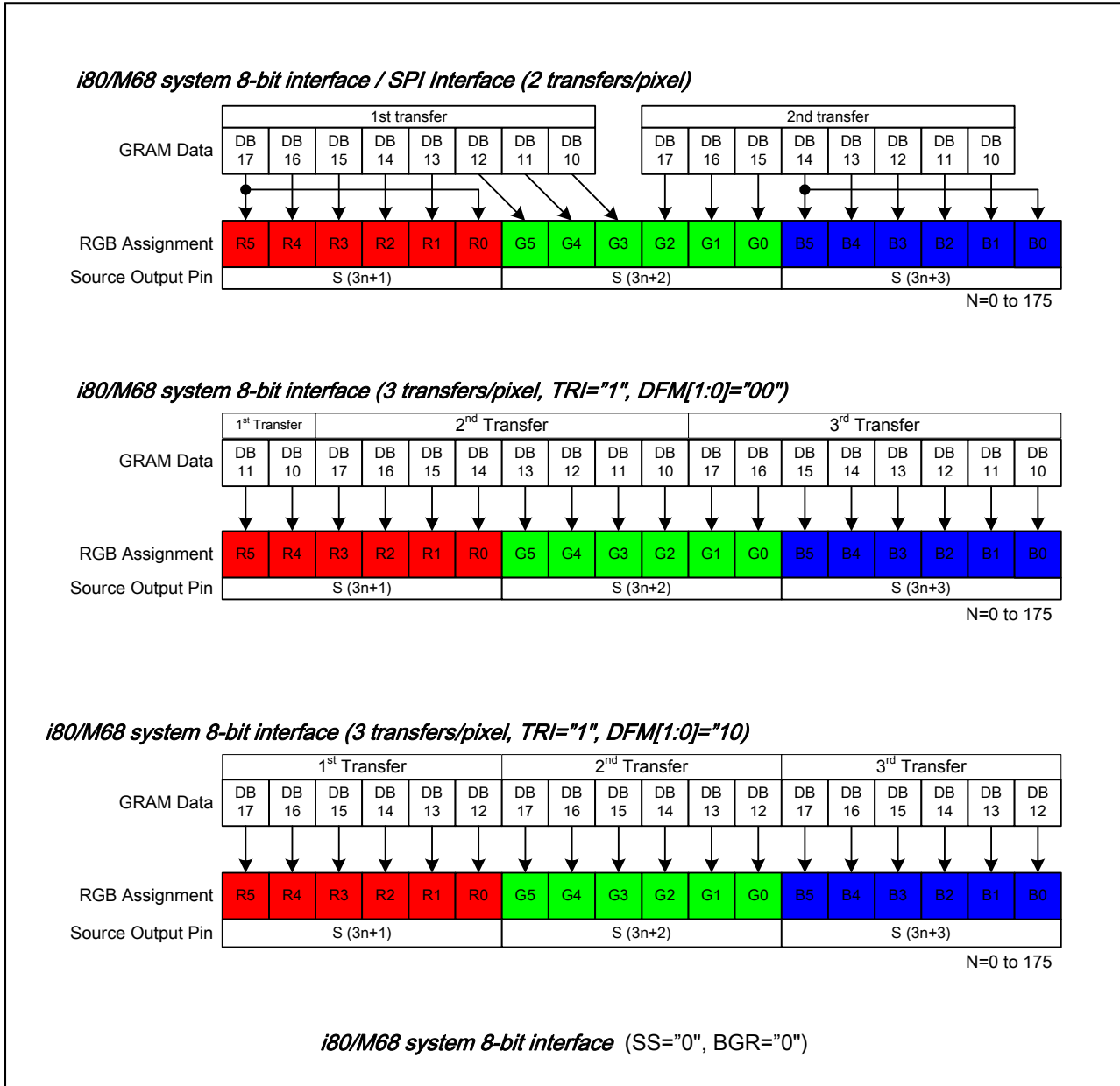
Figure32 i80-System Interface with 8-bit Data Bus (SS="0", BGR="0")
