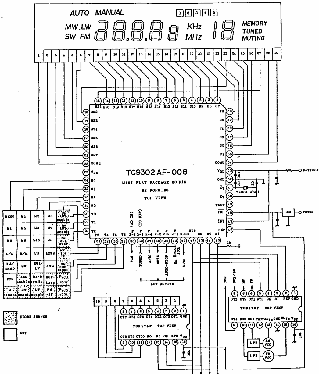
o TC9302AF-008 EXAMPLE OF APPLICATION CIRCUIT
