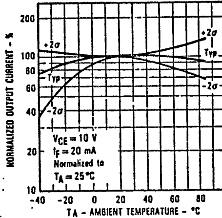
Normalized Output Current vs. Ambient Temperature
