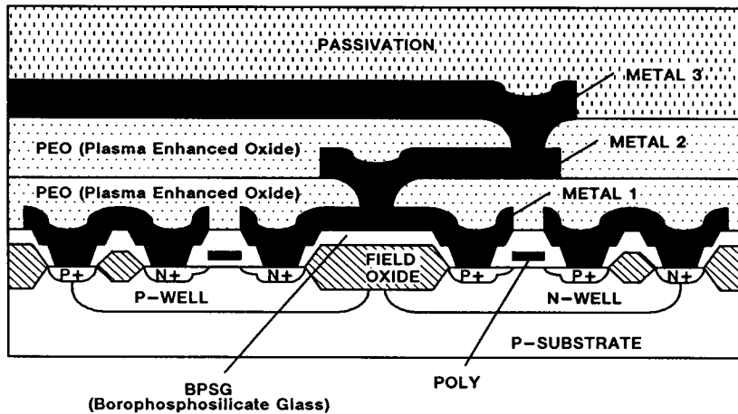
FIGURE 2 – Triple Layer Metal Cross Section
