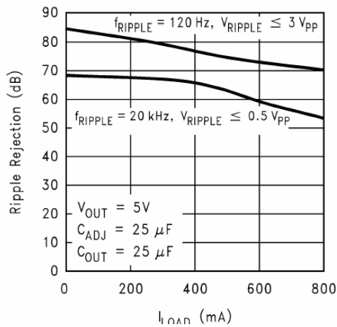
B1117-ADJ Ripple Rejection vs. Current
