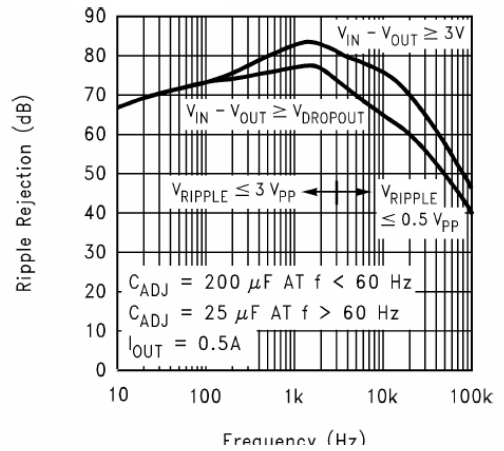
B1117-2.85 Ripple Rejection
