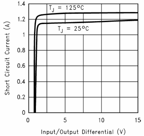
Short-Circuit Current
