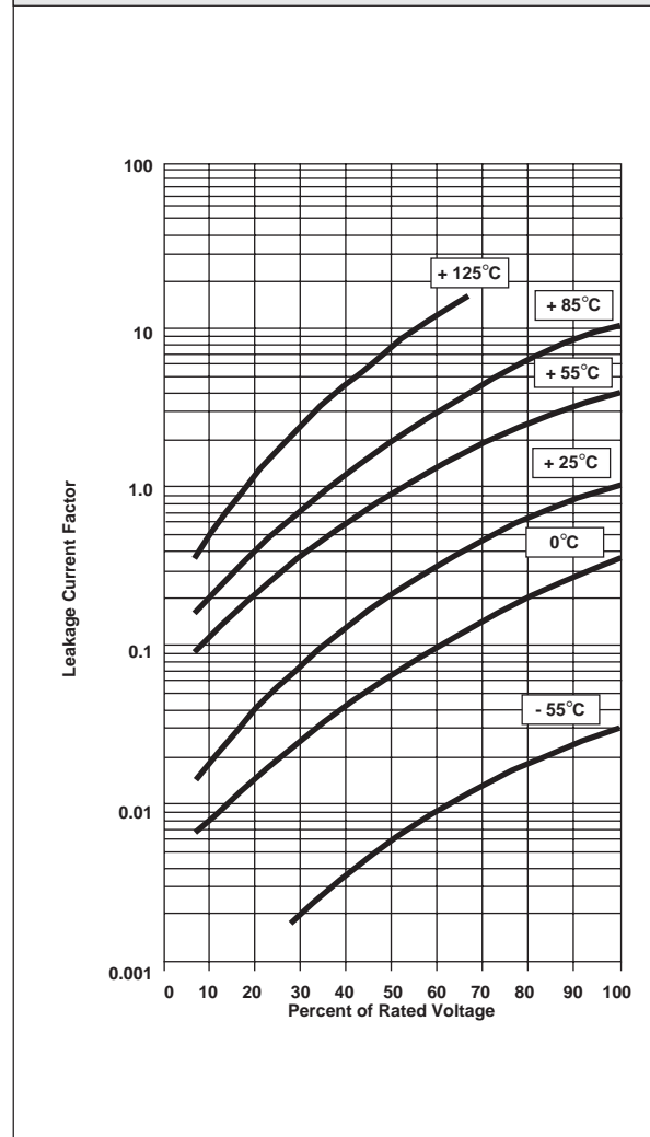
TYPICAL LEAKAGE CURRENT FACTOR RANGE
