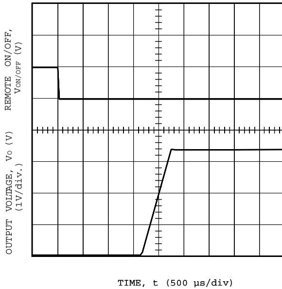
Figure 32. NH050F-L Typical Start-Up from Remote On/Off, V i = 5 V, I o = 15 A
