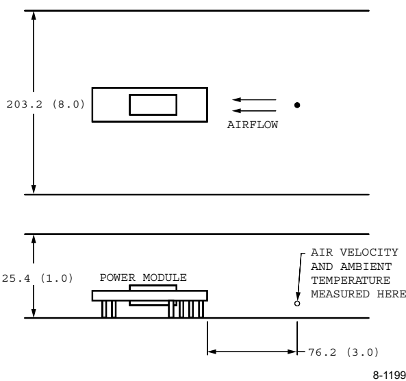
Figure 40. Thermal Test Setup
