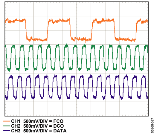
Figure 59. LVDS Output Timing Example in ANSI Mode (Default)
