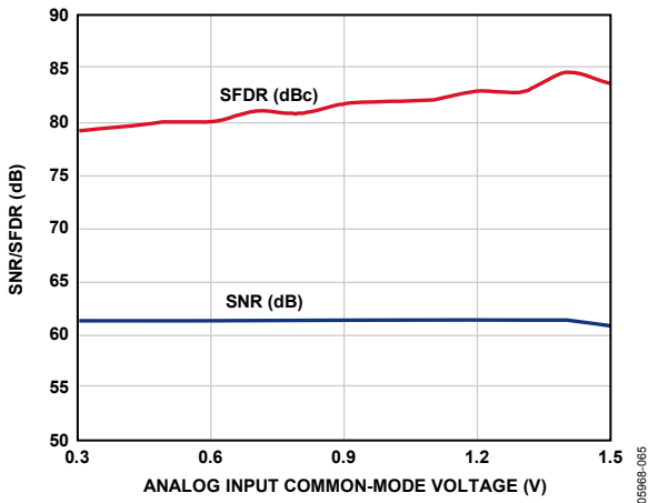
Figure 43. SNR/SFDR vs. Common-Mode Voltage, f_{IN} = 2.3 MHz, AD9212-40
