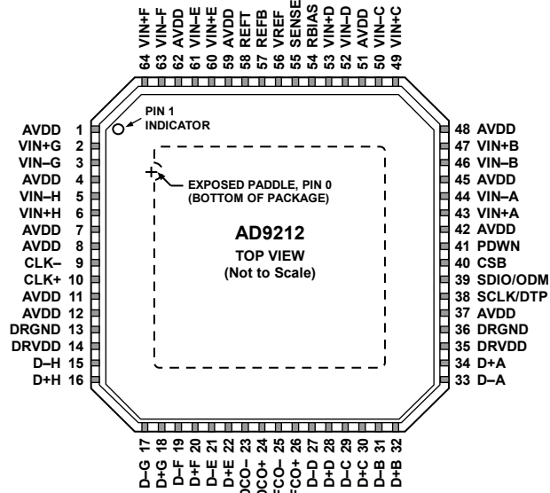
Figure 5. 64-Lead LFCSP Top View
