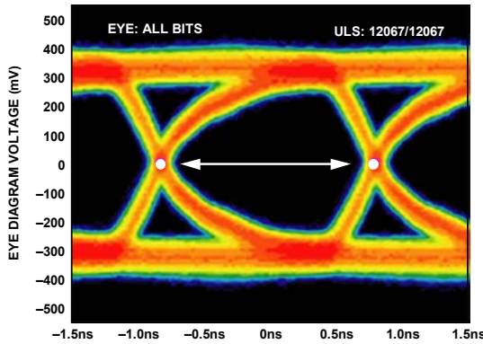
Figure 60. Data Eye for LVDS Outputs in ANSI Mode with Trace Lengths Less than 24 Inches on Standard FR-4
