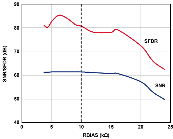
Figure 63. SNR/SFDR vs. RBIAS, AD9212-40
