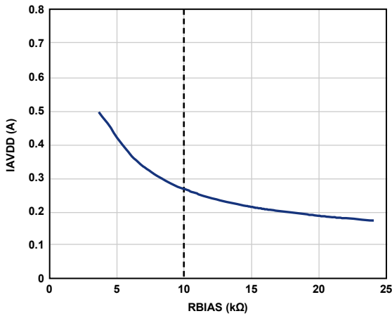
Figure 64. IAVDD vs. RBIAS, AD9212-40
