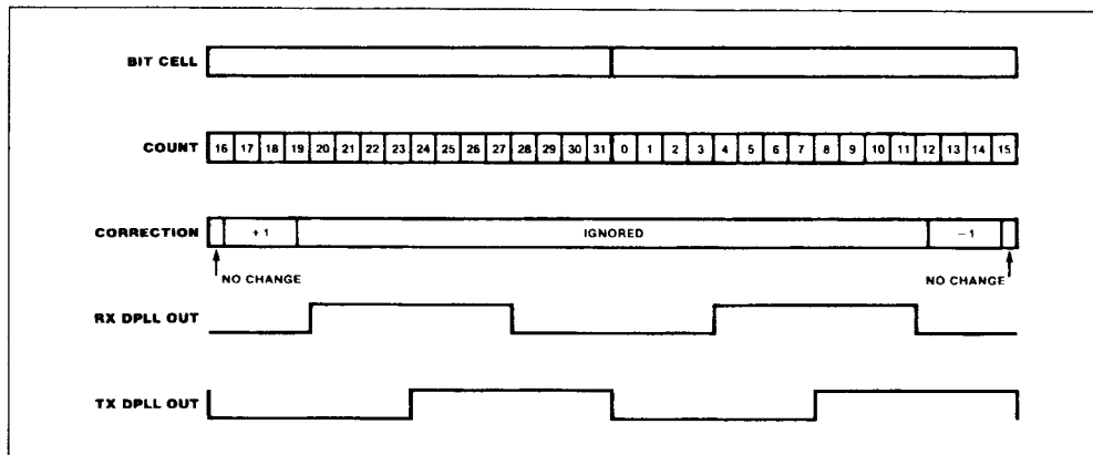
Figure 39 : DPLL in FM Mode.
