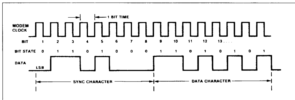
Figure 8 : Monosync Data Character Format.
