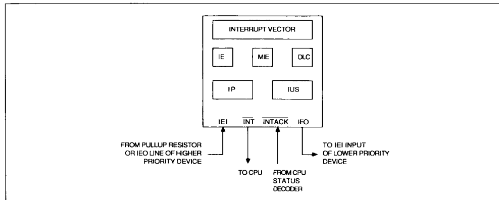
Figure 16 : Peripheral Interrupt Structure.
