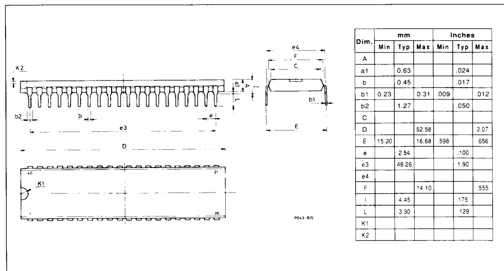
Figure 81: Z8530 40-Pin Dual in Line Plastic
