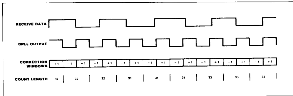
Figure 38 : DPLL Operating Example.
