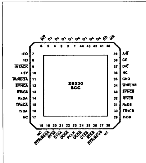
Figure 4 : Chip Carrier Pin Connection.
