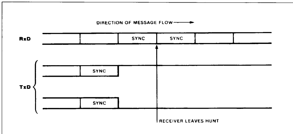
Figure 29 : Transmitter to Receiver Synchronization.
