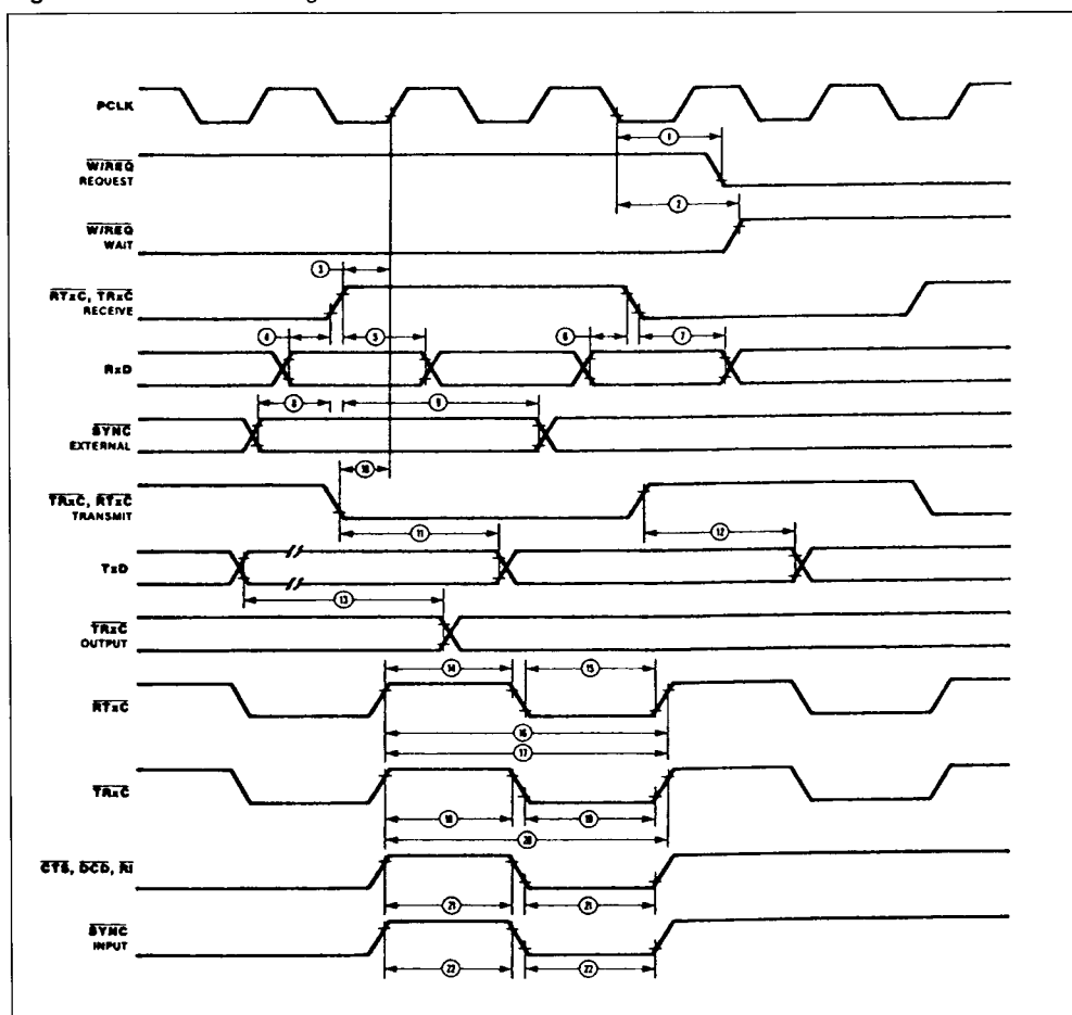
Figure 79 : General Timing.
