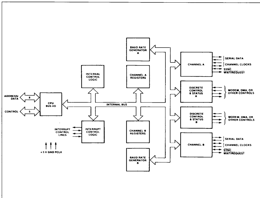
Figure 2 : SCC Block Diagram.
