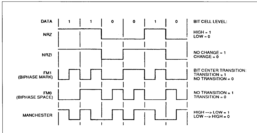
Figure 35 : Data Encoding Methods.
