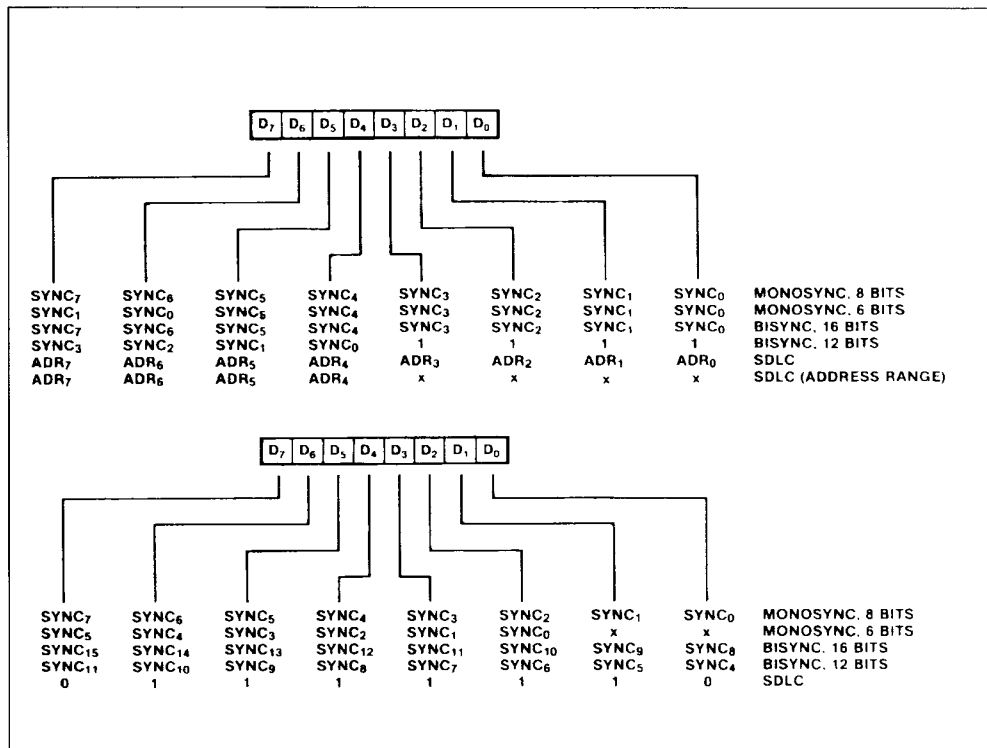
Figure 24 : Sync Character Programming.
