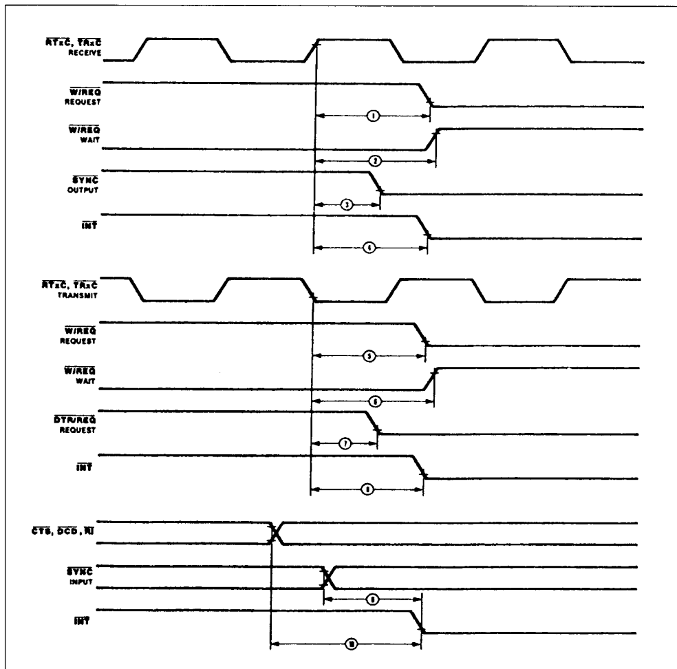
Figure 80 : System Timing.
