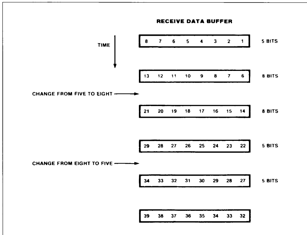
Figure 27 : Changing Character Length.
