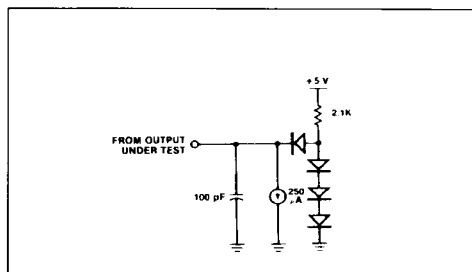
Figure 73 : Standard Test Load.
