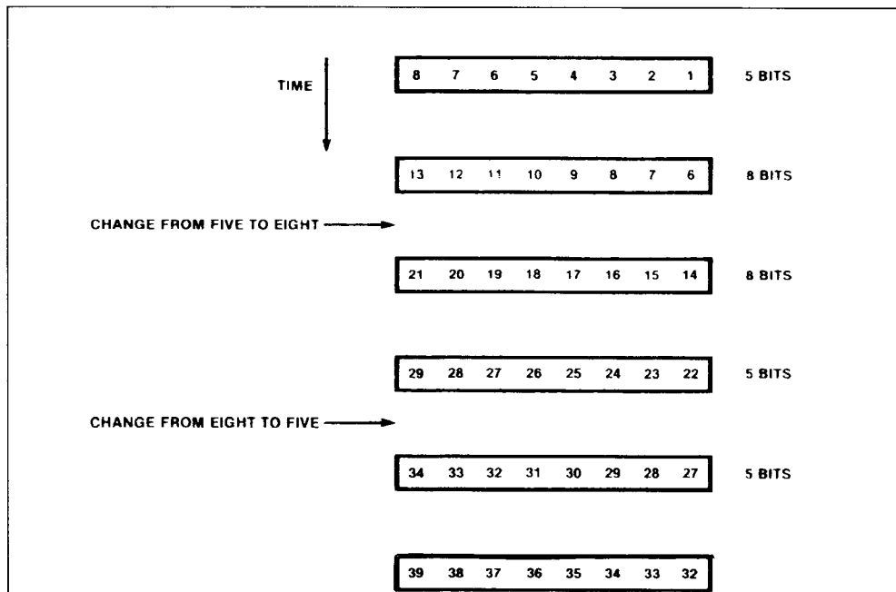
Figure 31 : Changing Character Length.
