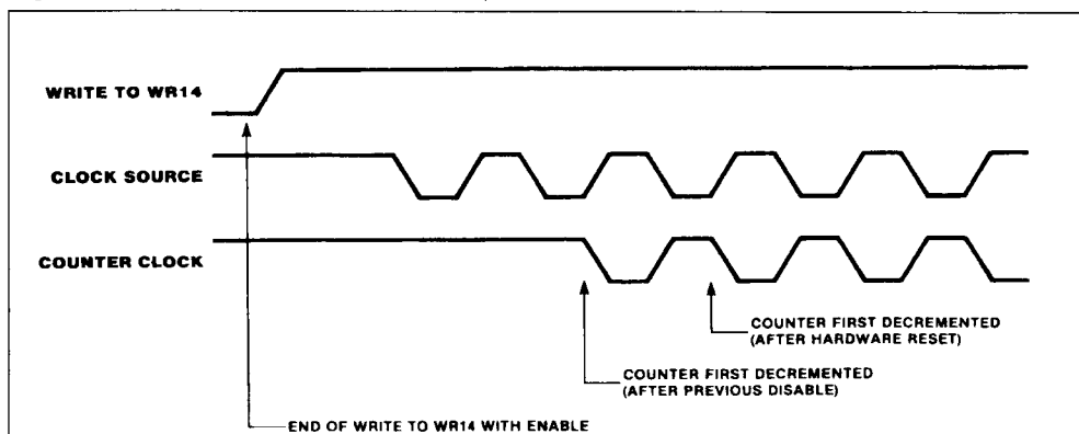
Figure 34 : Baud Rate Generator Start-Up.
