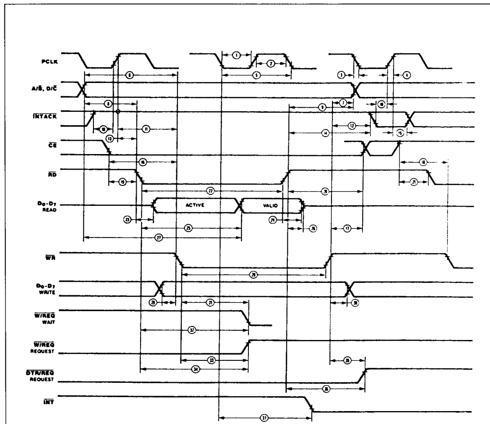
Figure 75 : Read and Write Timing.
