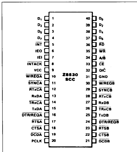
Figure 3 : DIP Pin Connections.
