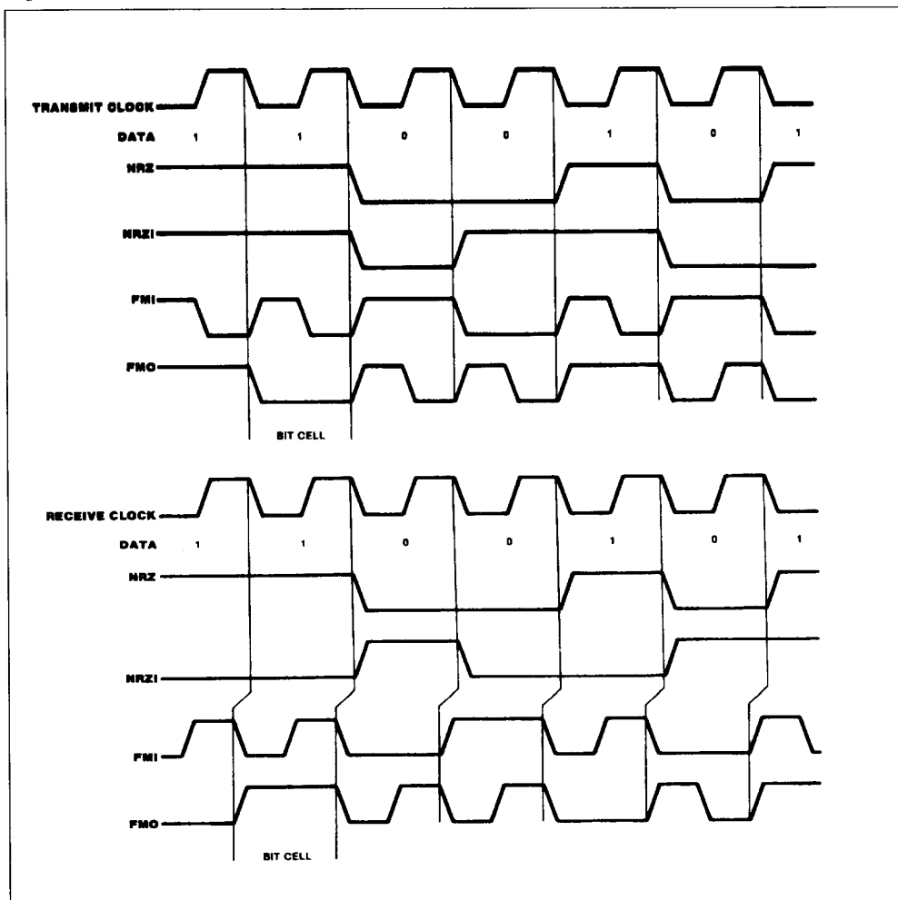
Figure 53 : NRZ(NRZI)FM1(FM0) Timing.
