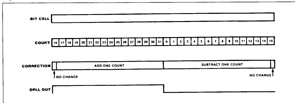
Figure 38 : DPLL Operating Example.
