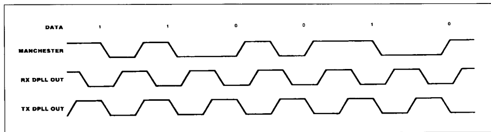
Figure 40 : Manchester Clock Recovery.
