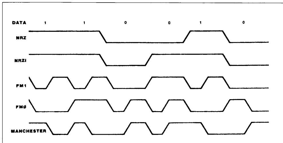
Figure 6 : Data Encoding Methods.
