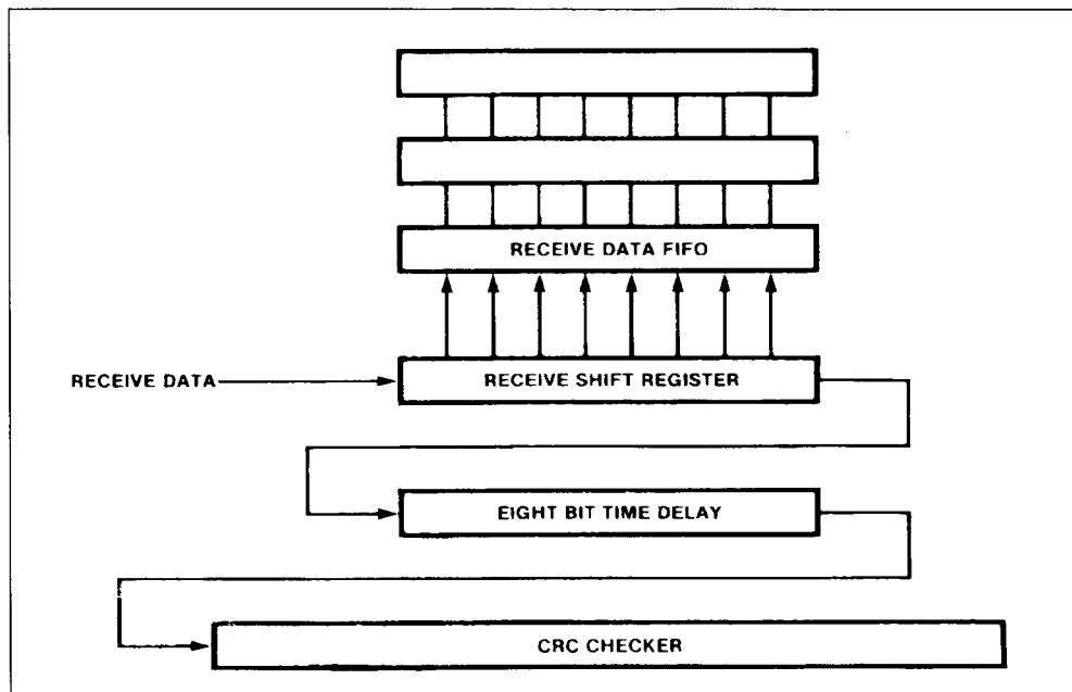
Figure 28 : Receive CRC Data Path.
