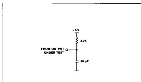
Figure 74 : Open-Drain Test Load.
