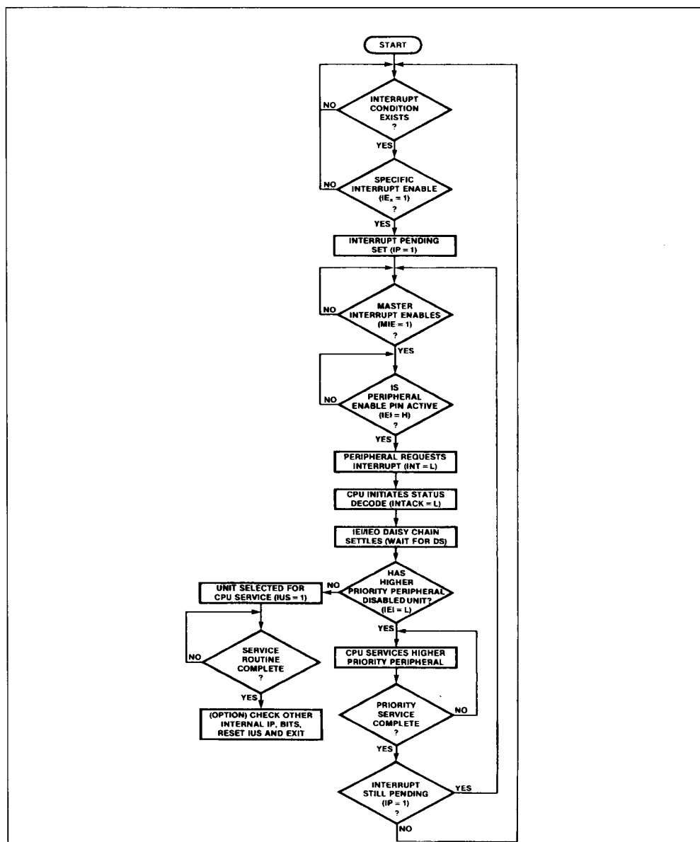
Figure 17 : Interrupt Flowchart.
