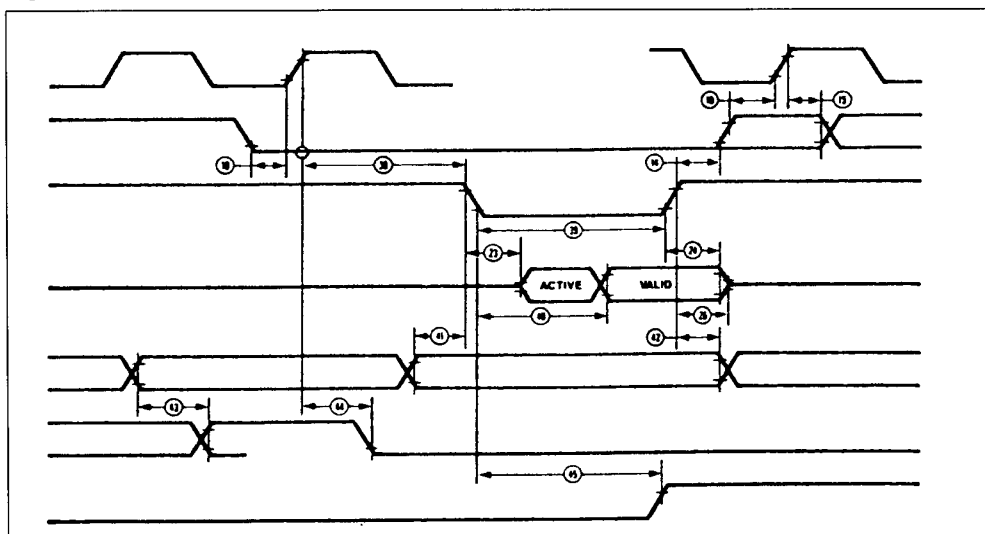
Figure 77 : Reset Timing.
