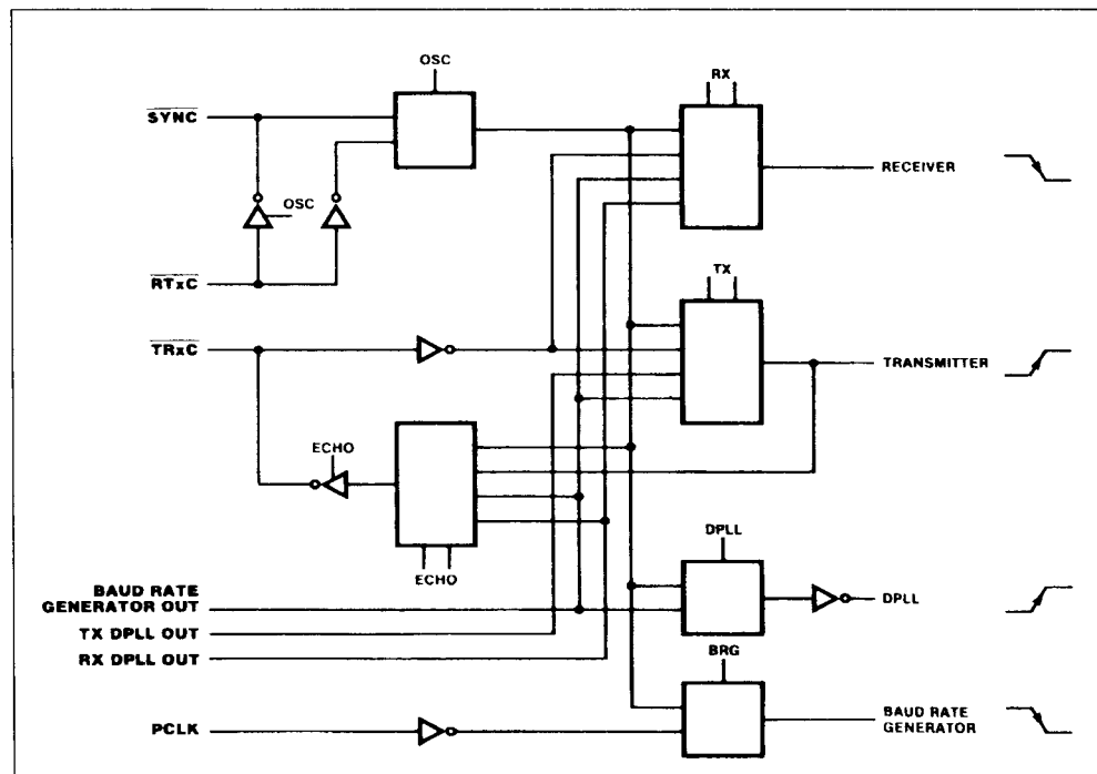
Figure 32 : Clock Multiplexer.
