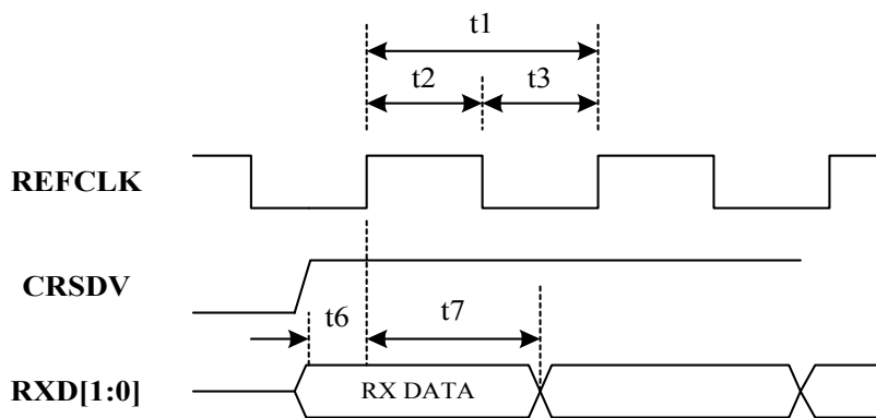
RMII Receive Timing
