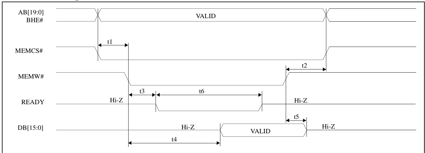
Figure 16: MEMW# Timing (Non-68000)
