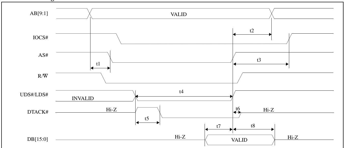
Figure 10: IOW# Timing (68000)
