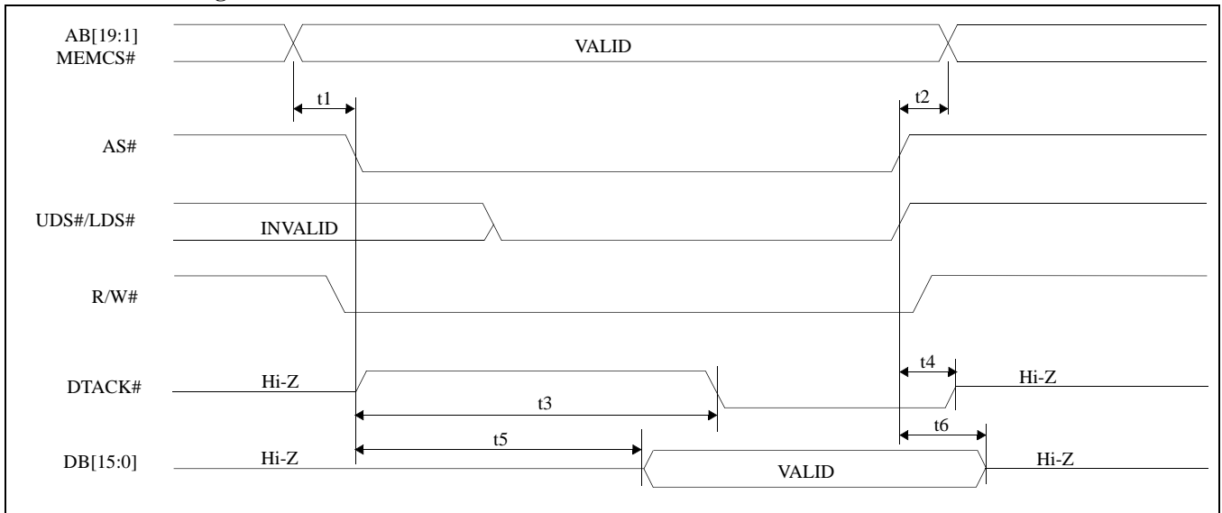
Figure 12: MEMW# Timing (68000)
