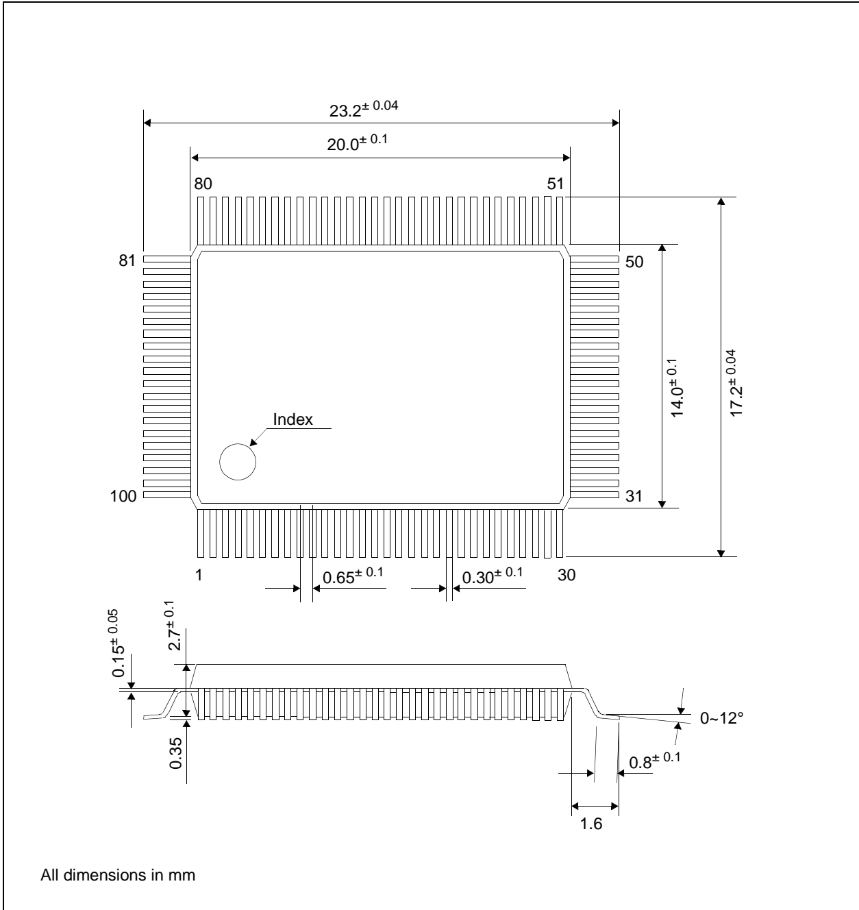
Figure 37: Mechanical Drawing QFP5-100pin-S2
