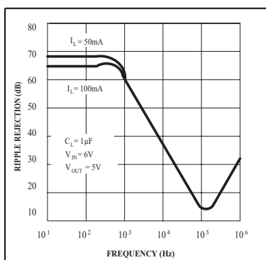
Ripple Rejection
