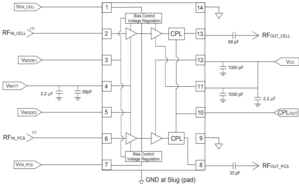
Figure 3: Application Circuit
