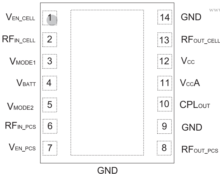
Figure 2: Pinout
