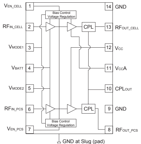
Figure 1: Block Diagram www.DataSheet4U.com
