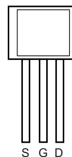
TO-92 (front view)
