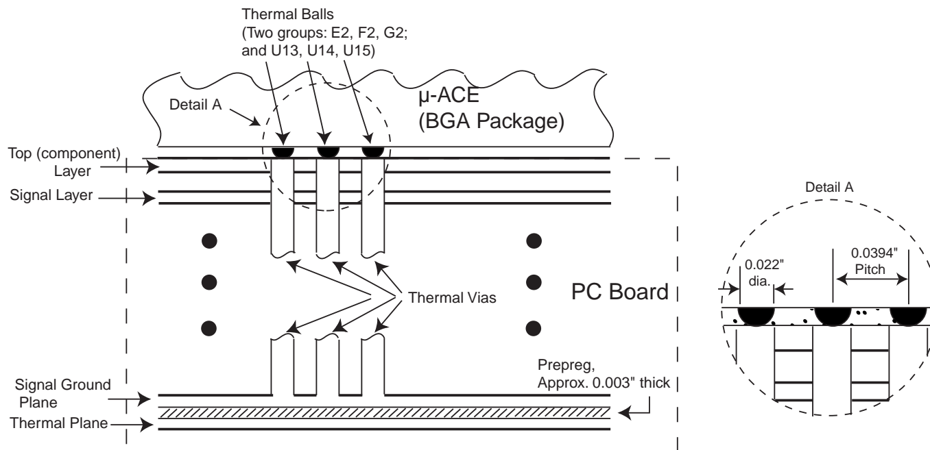
FIGURE 17. THERMAL DESIGN FOR \mu -ACE (BGA PACKAGES)
