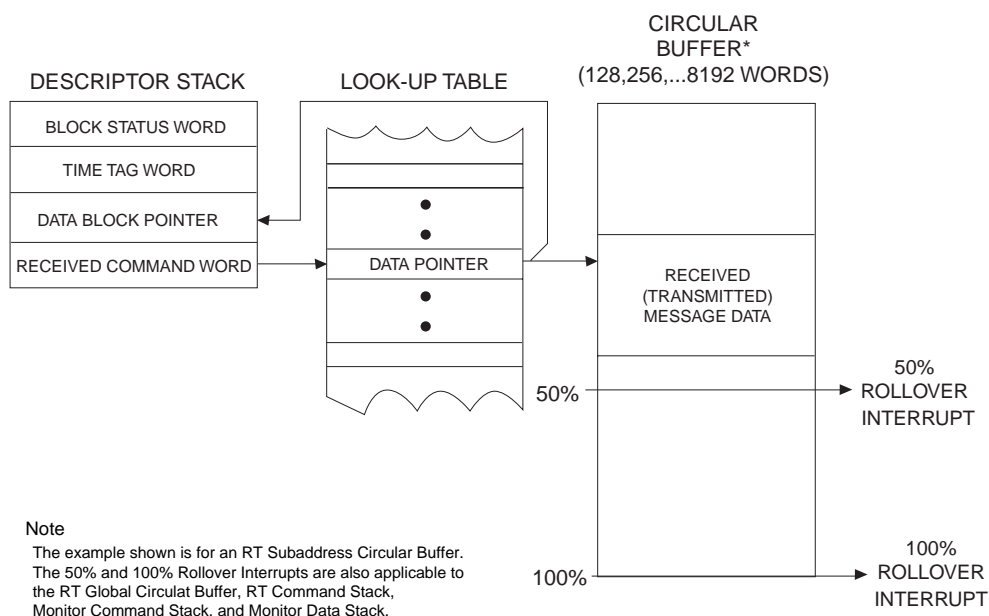
FIGURE 9. 50% and 100% ROLLOVER INTERRUPTS
