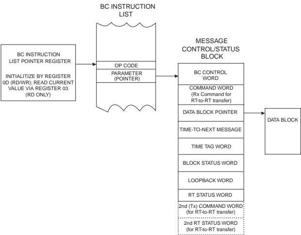
FIGURE 2. BC MESSAGE SEQUENCE CONTROL
