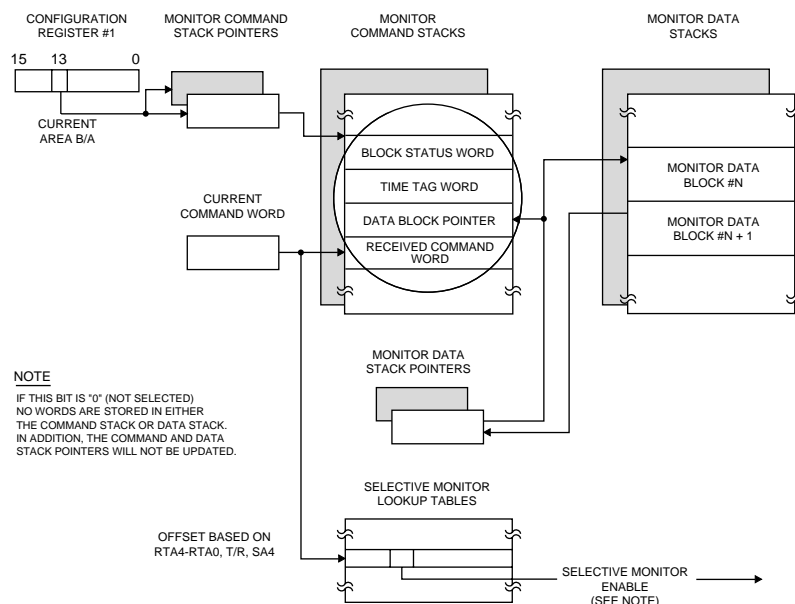
FIGURE 11. SELECTIVE MESSAGE MONITOR MEMORY MANAGEMENT
