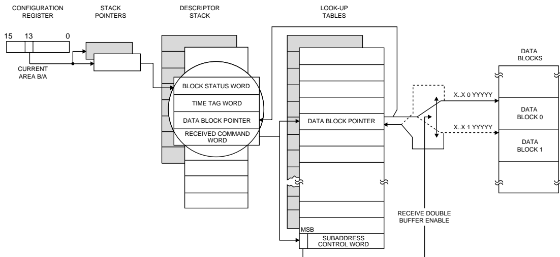
FIGURE 7. RT DOUBLE BUFFERED MODE
