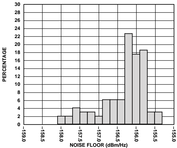
Figure 27. 20 MHz Offset Noise Floor Distribution at F_{LO} = 2140 MHz (BB Inputs at a Bias of 400 mV with no AC signal, T_A = 25^\circ\text{C} )
