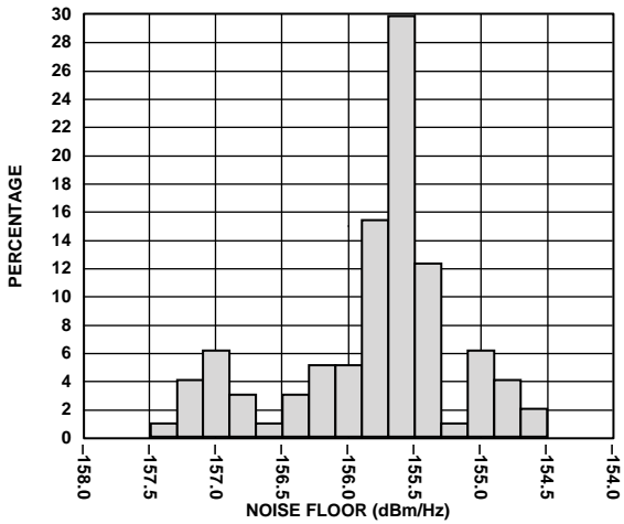
Figure 26. 20 MHz Offset Noise Floor Distribution at F_{LO} = 1900 MHz (BB Inputs at a Bias of 400 mV with no AC signal, T_A = 25^\circ\text{C} )
