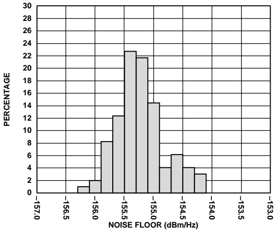
Figure 25. 20 MHz Offset Noise Floor Distribution at F_{LO} = 900 MHz (BB Inputs at a Bias of 400 mV with no AC signal, T_A = 25^\circ\text{C} )
