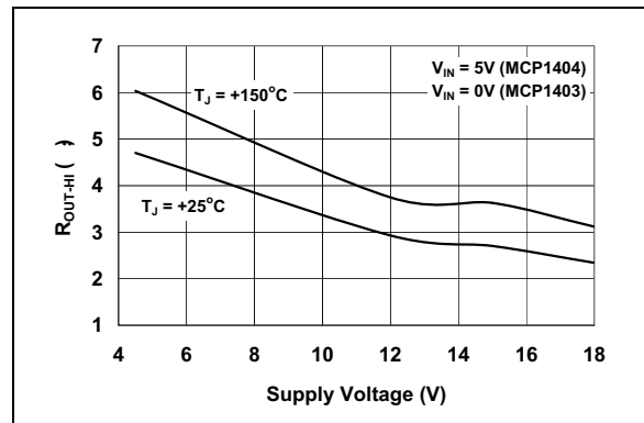
FIGURE 2-11: Output Resistance (Output High) vs. Supply Voltage.
