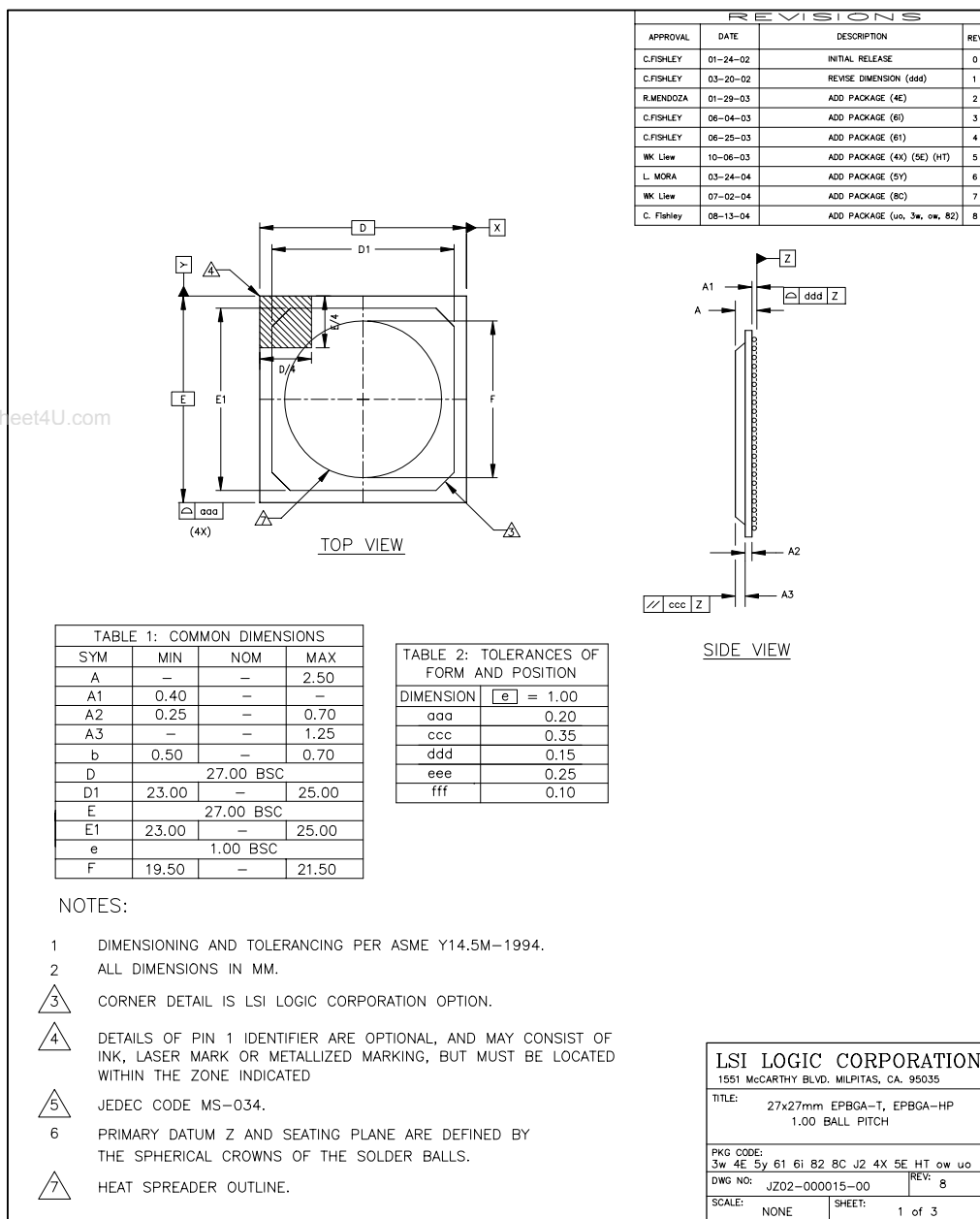
Figure 5 JZ02-000015-00 (5Y) Mechanical Drawing (Sheet 1 of 3)
