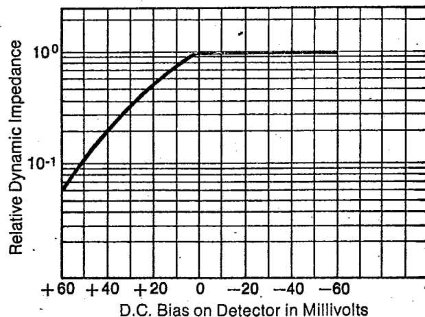
Fig. 3 — Dynamic impedance of the InSb detector is reduced by a positive bias that can be generated by background.
