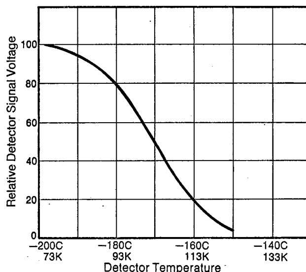
Fig. 5 — Relative signal voltage vs. operating temperature.
