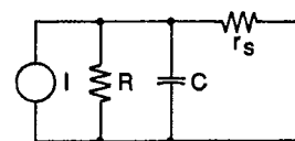
Fig. 4 — Equivalent circuit of the InSb detector.
