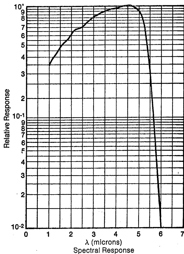
Fig. 1 — Spectral response of InSb detector peaks at 4.5 \mu\text{m} in usable range from 1 to 5.5 \mu\text{m} in the near infrared.
