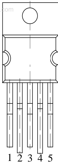
5-Lead TO-220(B)
