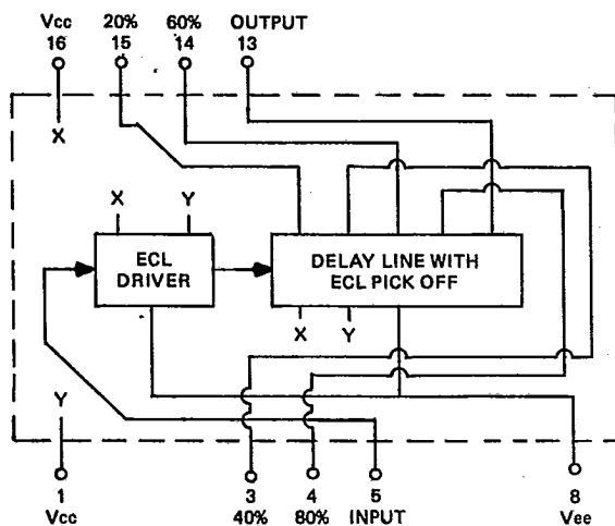
SCHEMATIC
