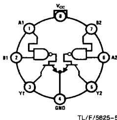
Top View Pin 4 is in electrical contact with the case. Order Number DS55461H or DS75461H
