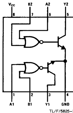
Top View Order Number DS55463J-8, DS75463J-8 or DS75463N See NS Package Numbers J08A or N08E
