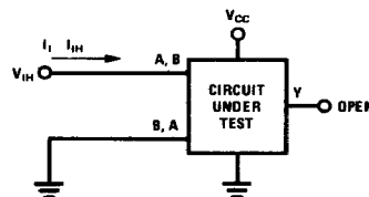
FIGURE 3. I_I , I_{IH}
