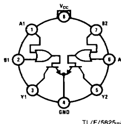
Top View Pin 4 is in electrical contact with the case. Order Number DS55464H or DS75464H
