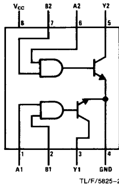
Top View Order Number DS55462J-8, DS75462J-8 or DS75462N See NS Package Numbers J08A or N08E
