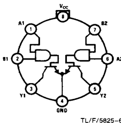
Top View Pin 4 is in electrical contact with the case. Order Number DS55462H or DS75462H See NS Package Number H08C
