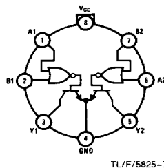
Top View Pin 4 is in electrical contact with the case. Order Number DS55463H or DS75463H See NS Package Number H08C
