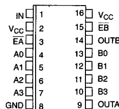
DS1045S 16-PIN SOIC (300 MIL) See Mech. Drawings Section
