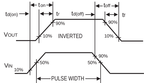
Figure 18. Switching Waveforms
