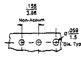
Recommended P.C. Board Hole Dimensions
