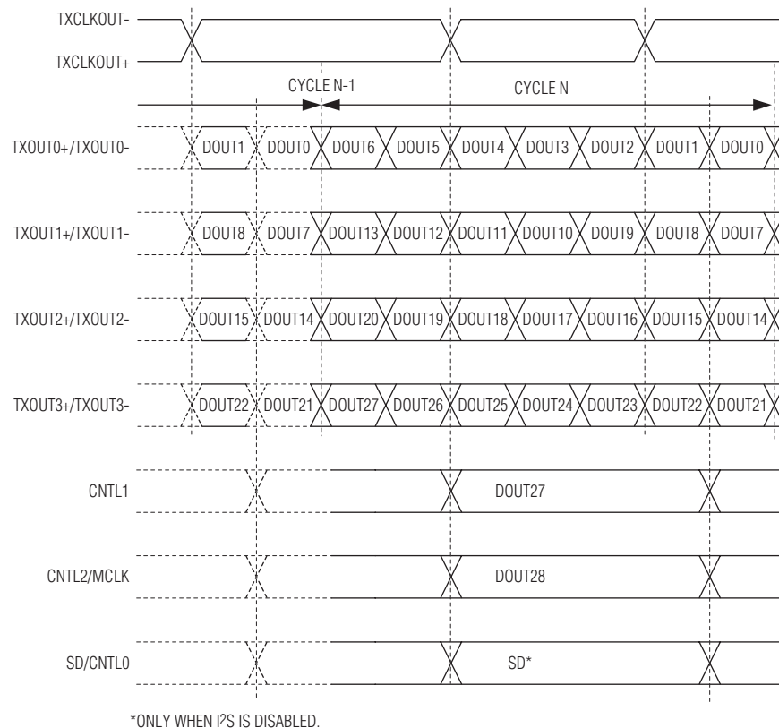
Figure 12. LVDS Output Timing
