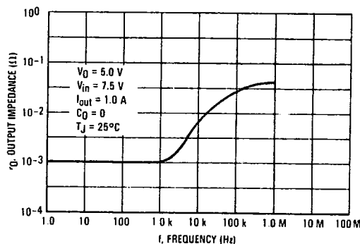
FIGURE 4 — OUTPUT IMPEDANCE
