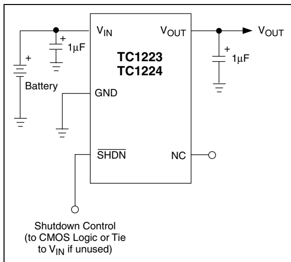
FIGURE 3-1: TYPICAL APPLICATION CIRCUIT
