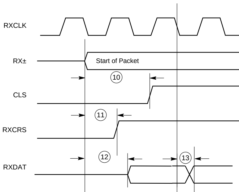
Figure 3. 10 Mbps Receive Start of Packet Timing (GPSI)
