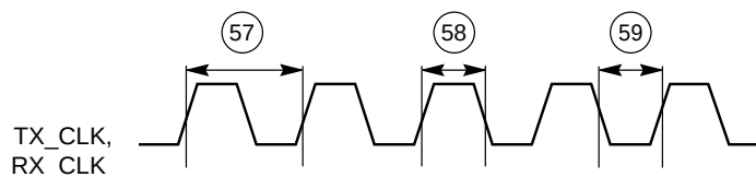
Figure 12. 10 Mbps Transmit and Receive Clock Timing (MII)
