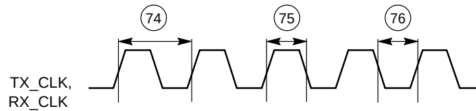
Figure 15. 1 Mbps HomePNA Clock Timing (MII)
