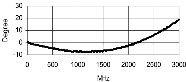
Phase Unbalance
