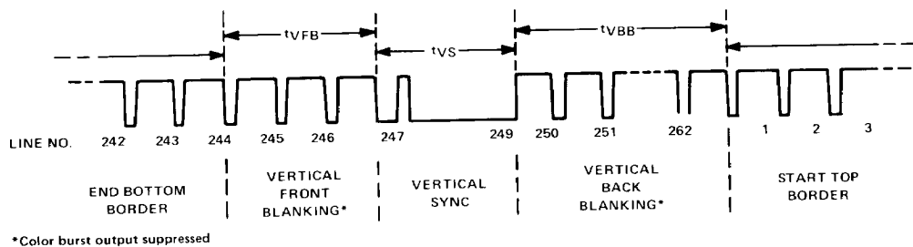
FIGURE 4-9 – TMS9118/9128 VERTICAL TIMING
