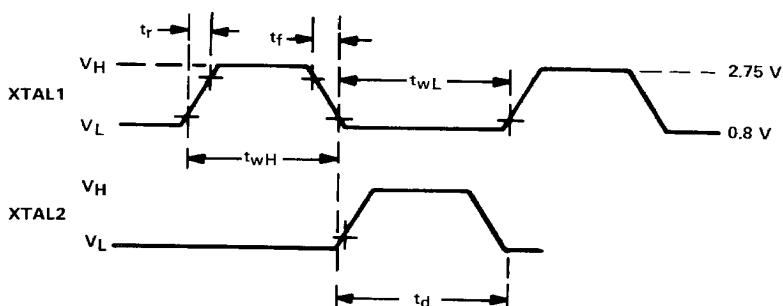
FIGURE 4-5 – EXTERNAL CLOCK TIMING WAVEFORM
