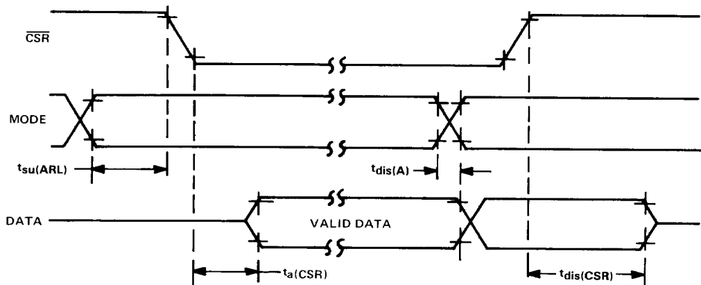
FIGURE 4-4 – CPU-VDP READ CYCLE FOR TMS9118/9128/9129
