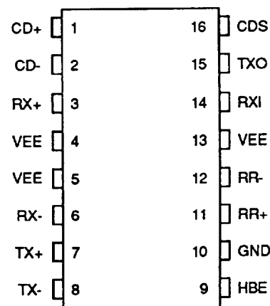
16-Pin DIP
