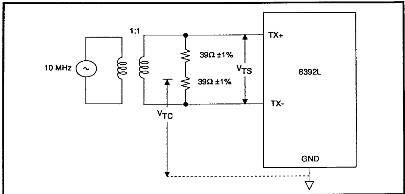
FIGURE 10: Test Circuit for TX± Input
