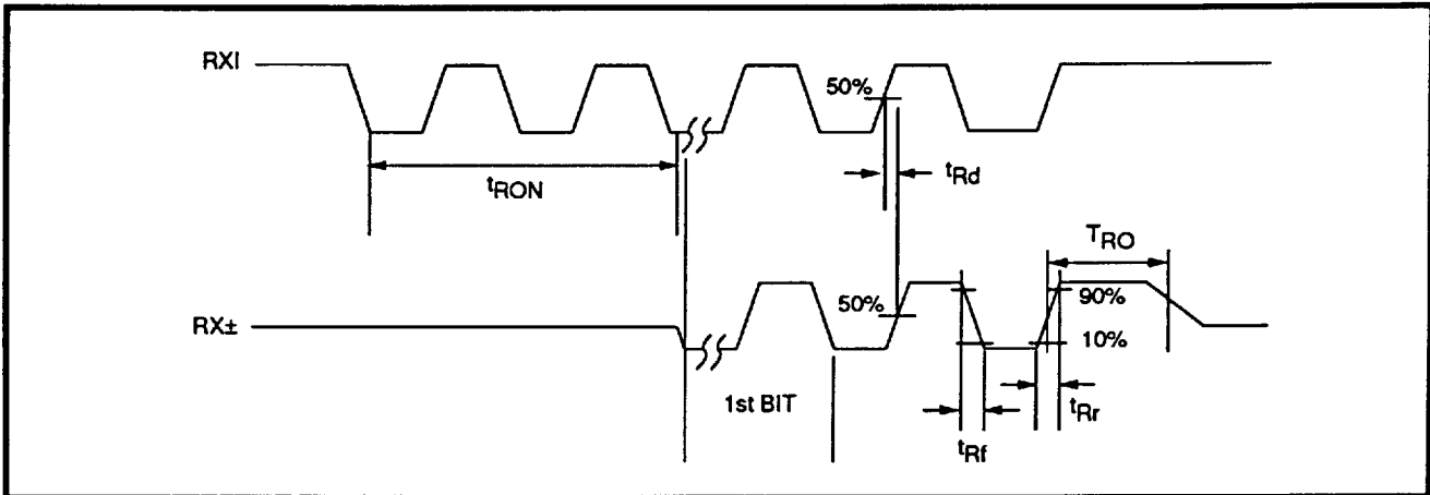
FIGURE 3: Receiver Timing
