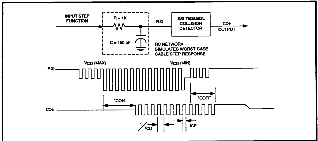
FIGURE 5: Collision Timing
