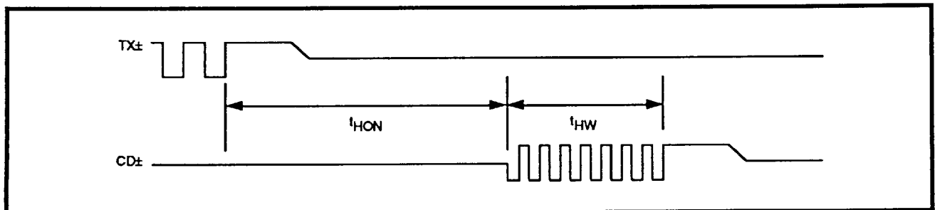
FIGURE 6: Heartbeat Timing
