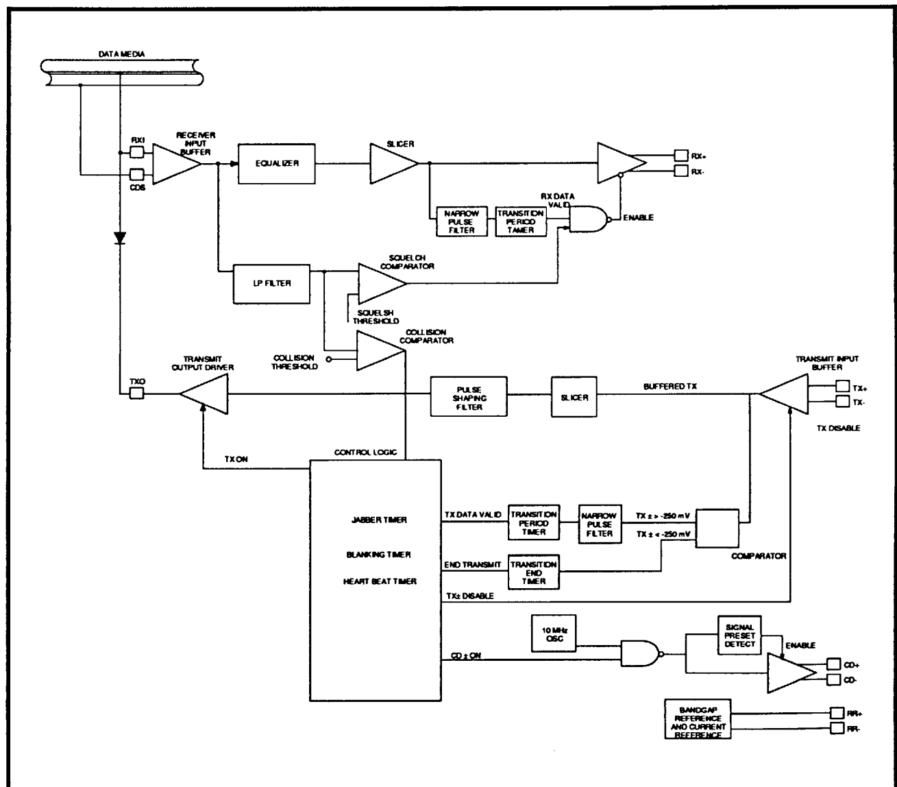
FIGURE 1: SSI 78Q8392L General System Block Diagram
