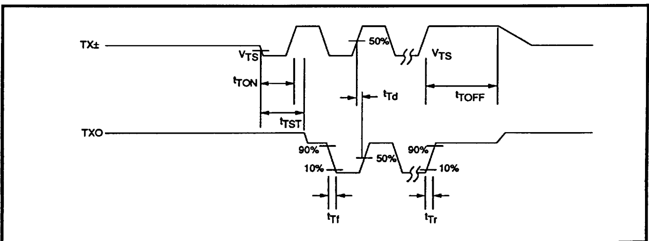
FIGURE 4: Transmitter Timing
