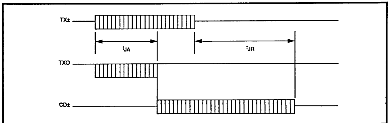
FIGURE 7: Jabber Timing
