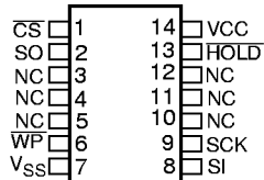
TSSOP Package (U14)
