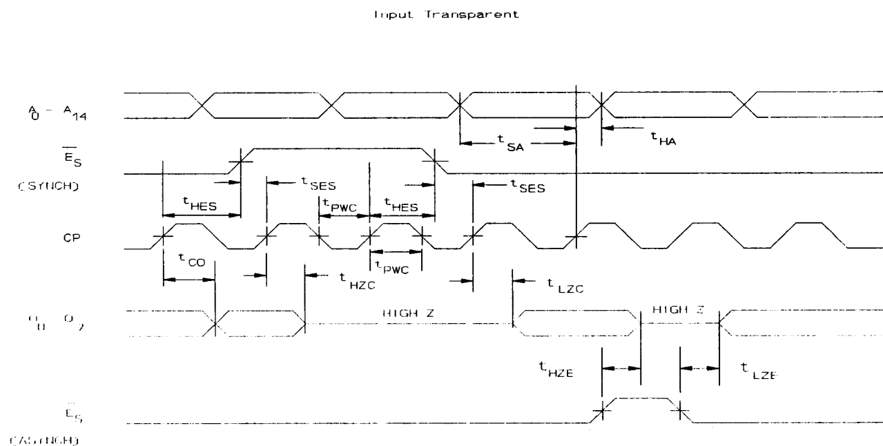
FIGURE 4. Switching waveforms.
