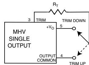
FIGURE 4: MHV SINGLE OUTPUT TRIM
