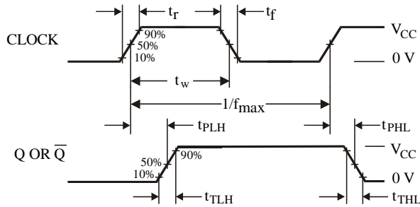
Figure 1. Switching Waveforms
