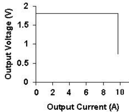
Fig 16. Output voltage vs current showing current limit point and converter shut down point
