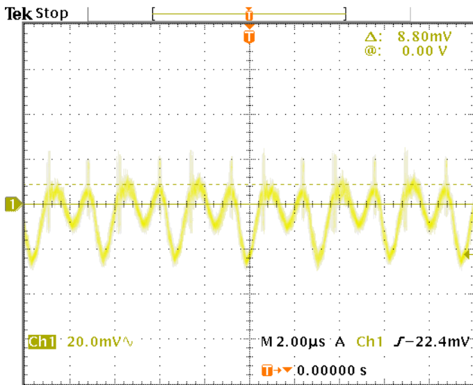
Fig 14. Output voltage Ripple & Noise at Vin=48v, Iout=5A Co=10μF tantalum capacitor + 1μF Ceramic capacitor, ch1: 20mV/div, time scale: 2μs/div.
