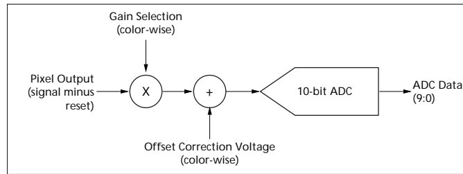
Figure 14: Black Level Calibration Flow Chart
