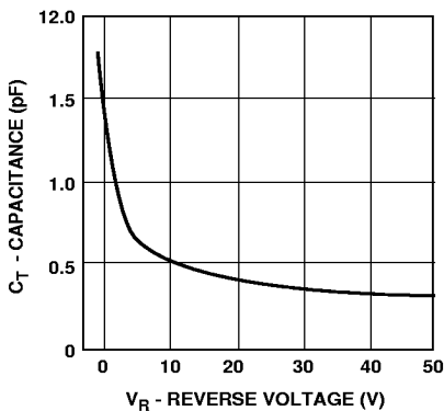
Figure 7. (5082-2800 or 1N5711) Typical Capacitance ( C_T ) vs. Reverse Voltage ( V_R ).
