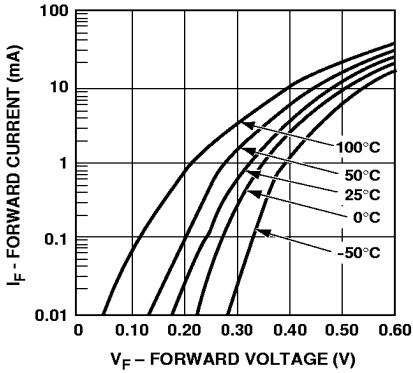
Figure 1. I-V Curve Showing Typical Temperature Variation for 5082-2300 Series and 5082-2900 Schottky Diodes.
