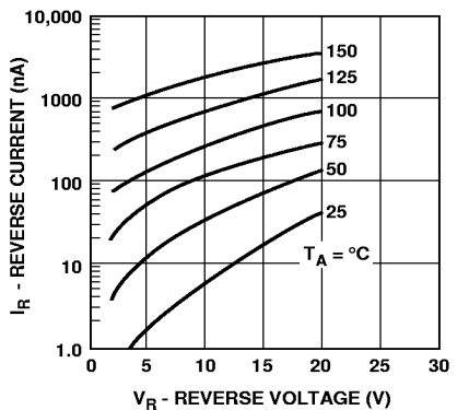
Figure 9. (5082-2810 or 1N5712) Typical Variation of Reverse Current ( I_R ) vs. Reverse Voltage ( V_R ) at Various Temperatures.
