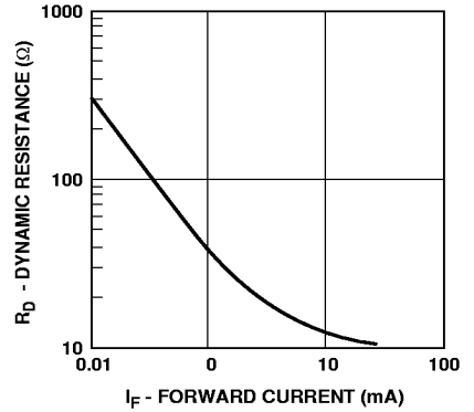
Figure 3. 5082-2300 Series and 5082-2900 Typical Dynamic Resistance ( R_D ) vs. Forward Current ( I_F ).
