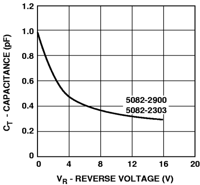
Figure 4. 5082-2300 and 5082-2900 Typical Capacitance vs. Reverse Voltage.
