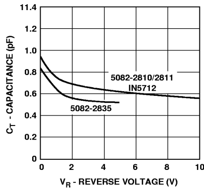
Figure 14. Typical Capacitance ( C_T ) vs. Reverse Voltage ( V_R ).
