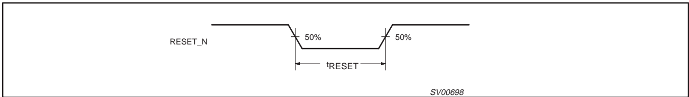
Figure 33. RESET_N Waveform
