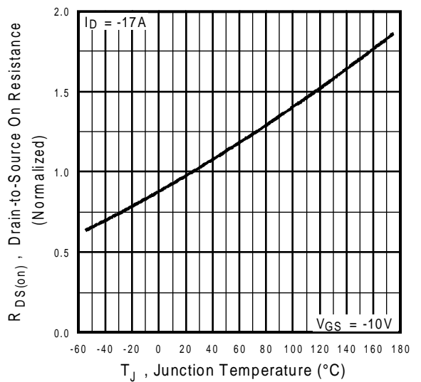
Fig 4. Normalized On-Resistance
