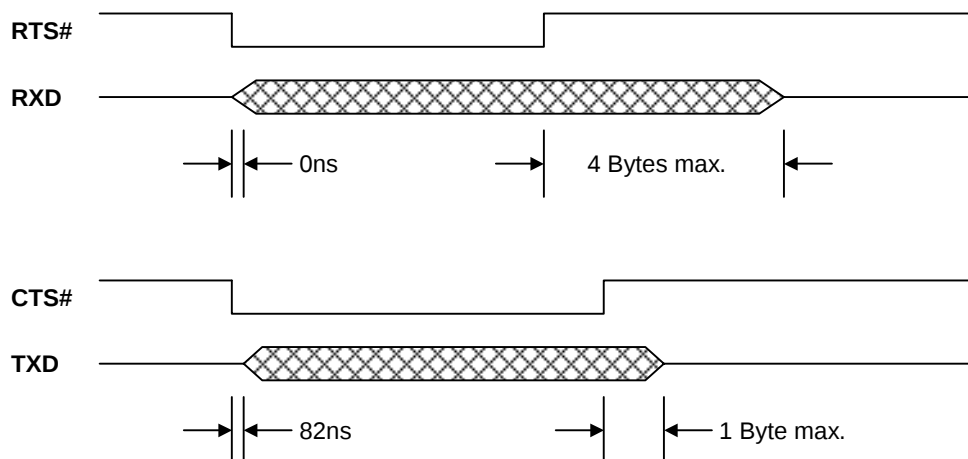
Figure 6-2: UART Timing Diagram
