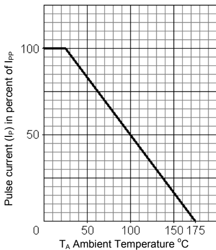
FIG. 4 Derating Curve
