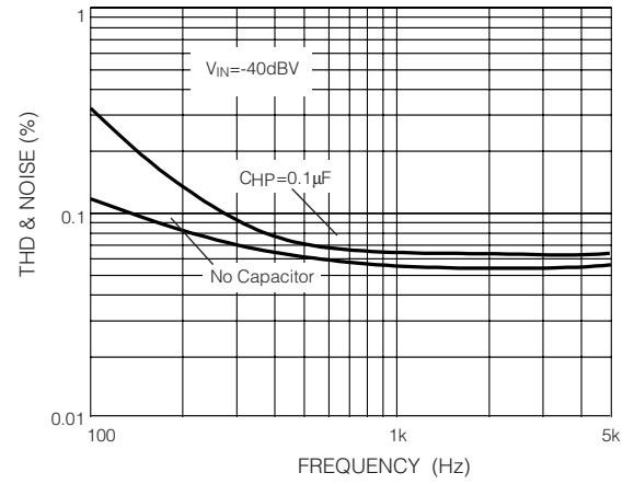
Fig. 12 THD & Noise vs Frequency
