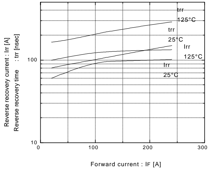
Reverse recovery characteristics t_{rr}, I_{rr} vs. I_F
