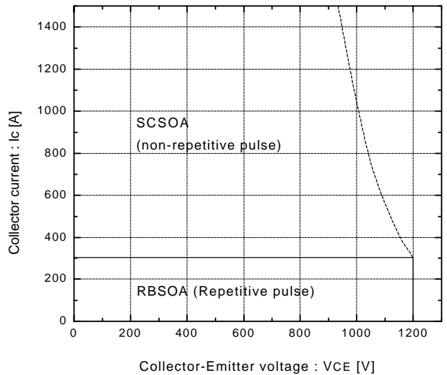
Reversed biased safe operating area +V_{GE}=15V, -V_{GE}\leq 15V, T_J\leq 125^\circ C, R_G\geq 5.6\Omega
